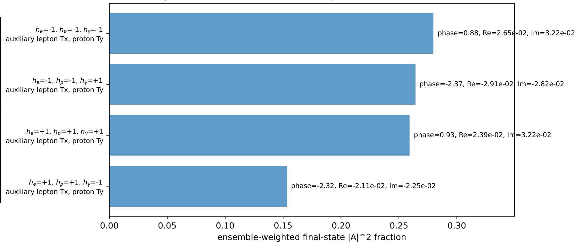
Leading initial-ensemble/final-state components (N=4, retained=95.6%)
