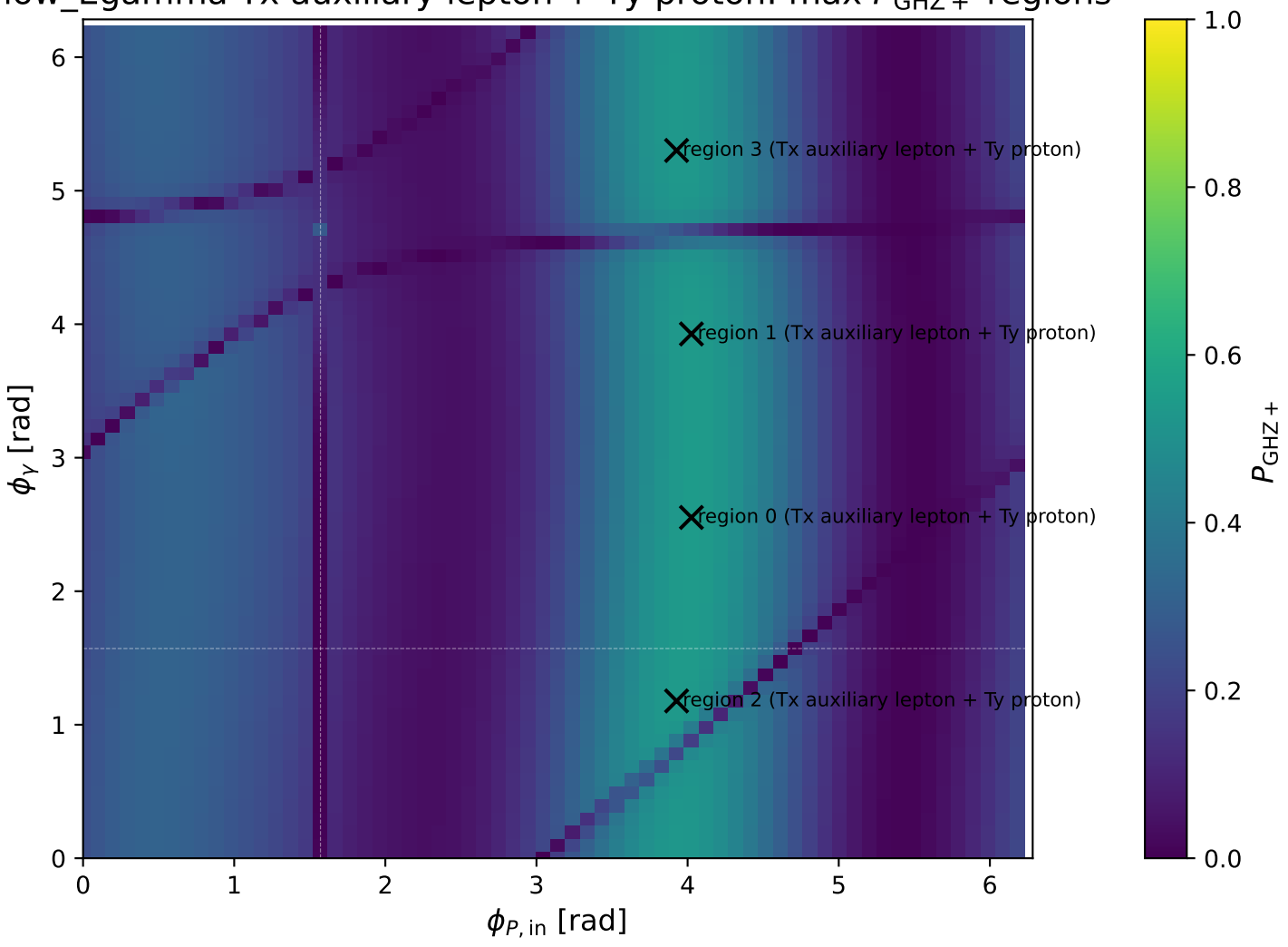
low_Egamma Tx auxiliary lepton + Ty proton: max P_{\text{GHZ}+} regions
