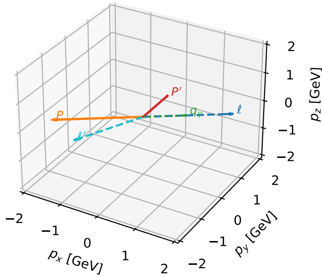
3D momenta
