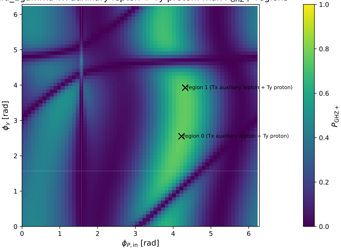
id_Egamma Tx auxiliary lepton + Ty proton: max P_{\text{GHZ}+} regions
