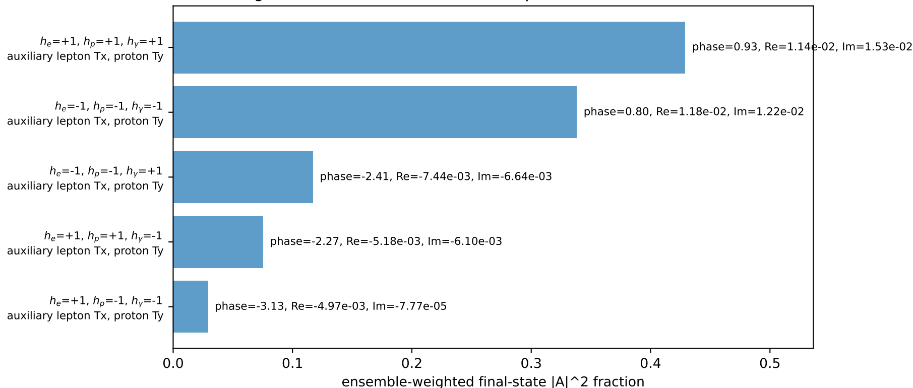
Leading initial-ensemble/final-state components (N=5, retained=98.9%)
