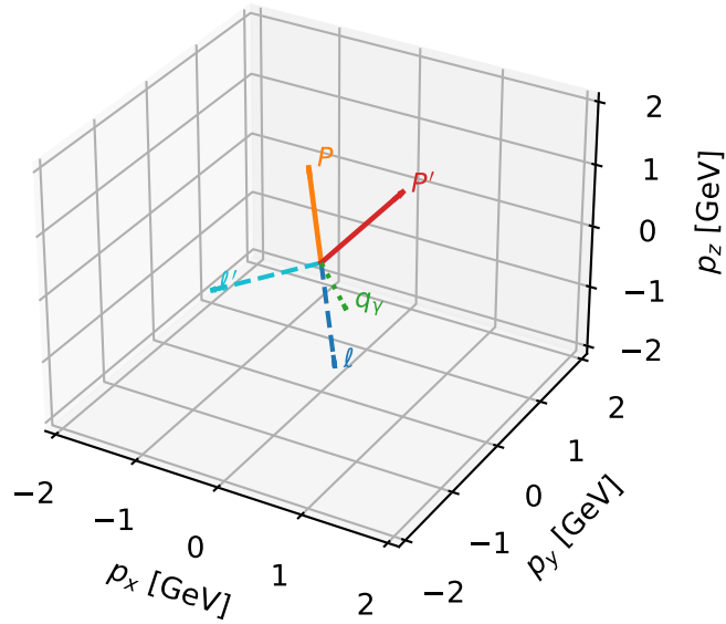
3D momenta
