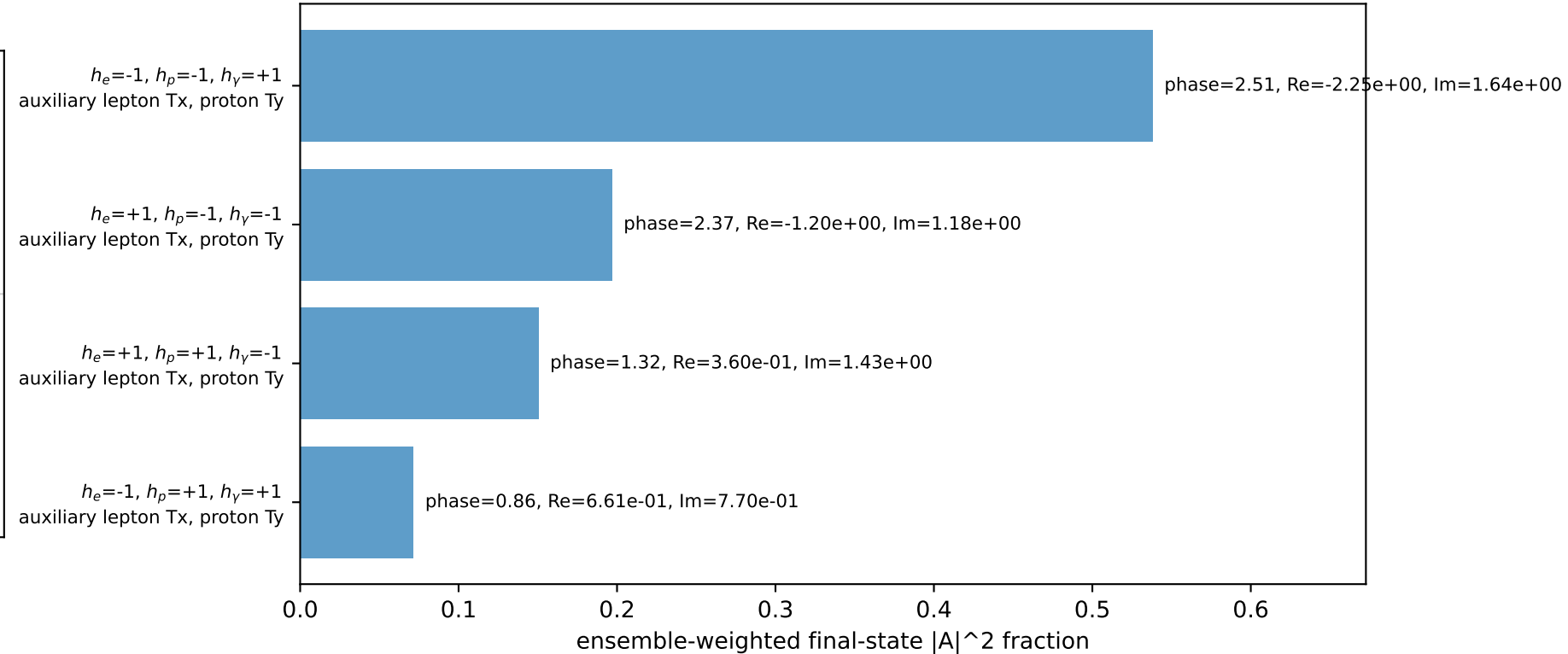
Leading initial-ensemble/final-state components (N=4, retained=95.7%)
