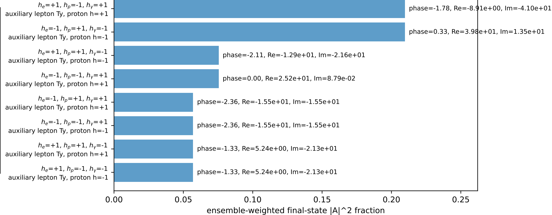
Leading initial-ensemble/final-state components (N=8, retained=79.8%)
