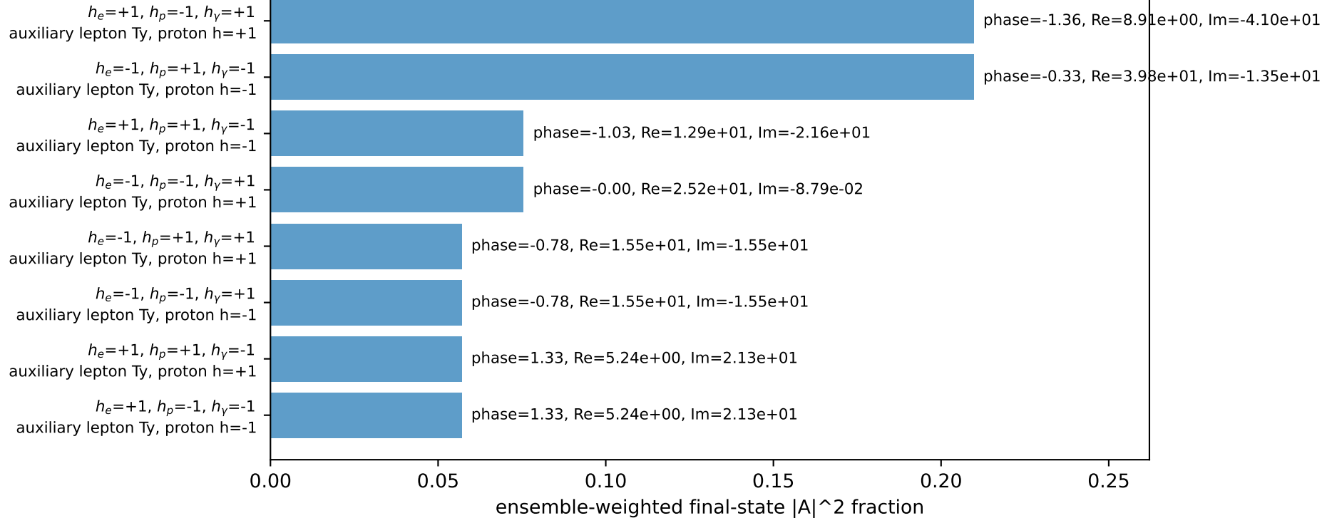
Leading initial-ensemble/final-state components (N=8, retained=79.8%)
