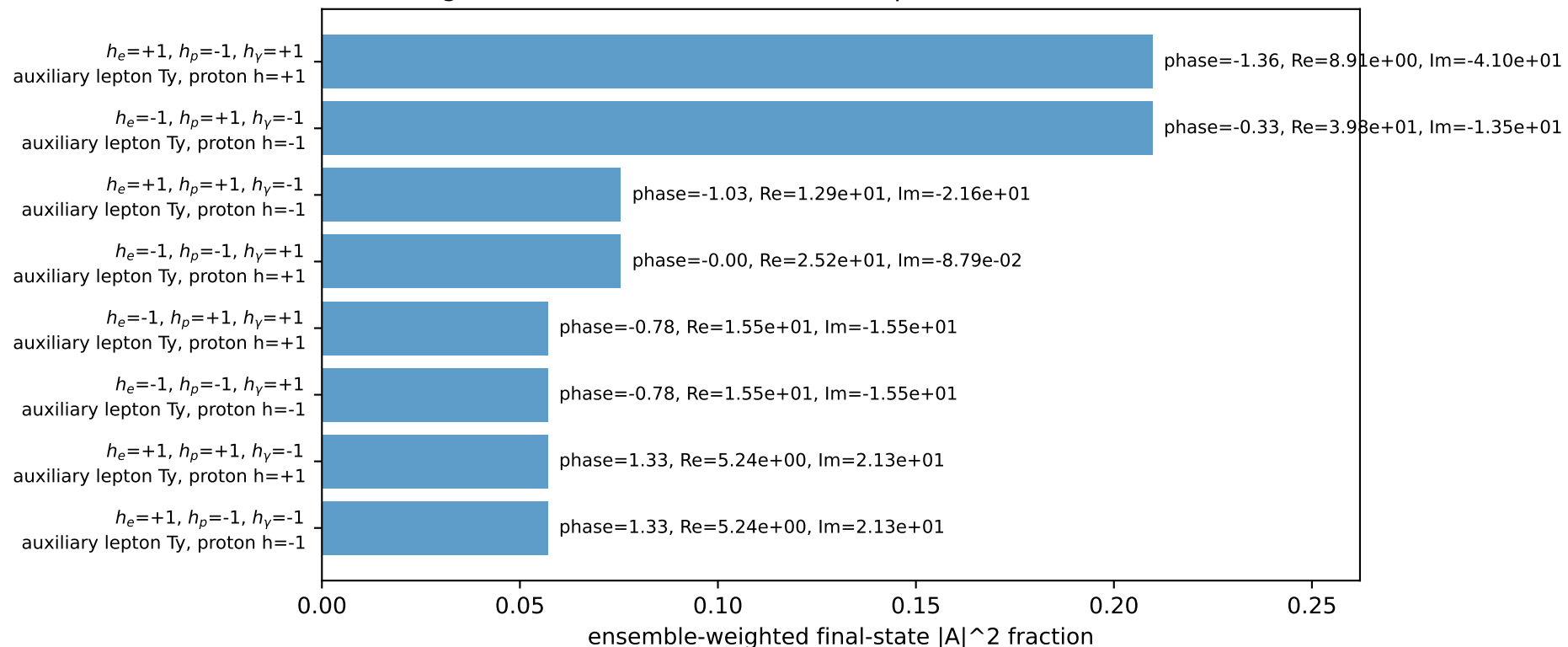
Leading initial-ensemble/final-state components (N=8, retained=79.8%)
