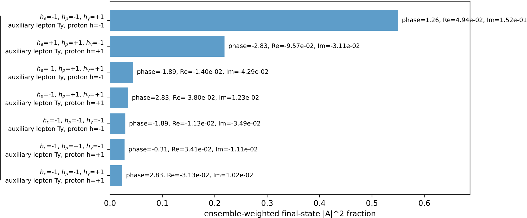
Leading initial-ensemble/final-state components (N=7, retained=92.7%)
