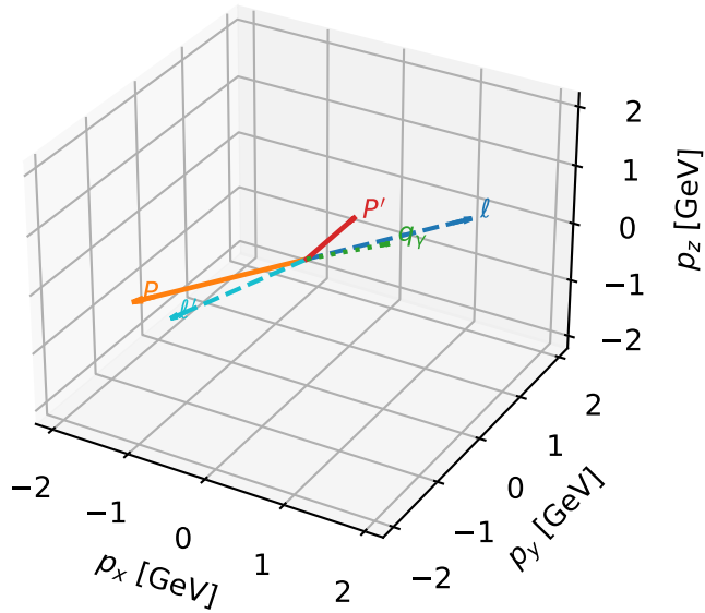
3D momenta
