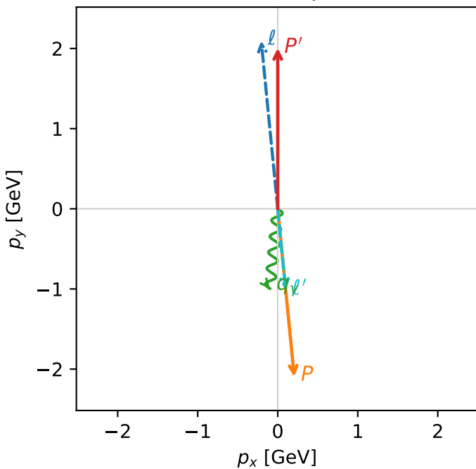
Transverse plane
