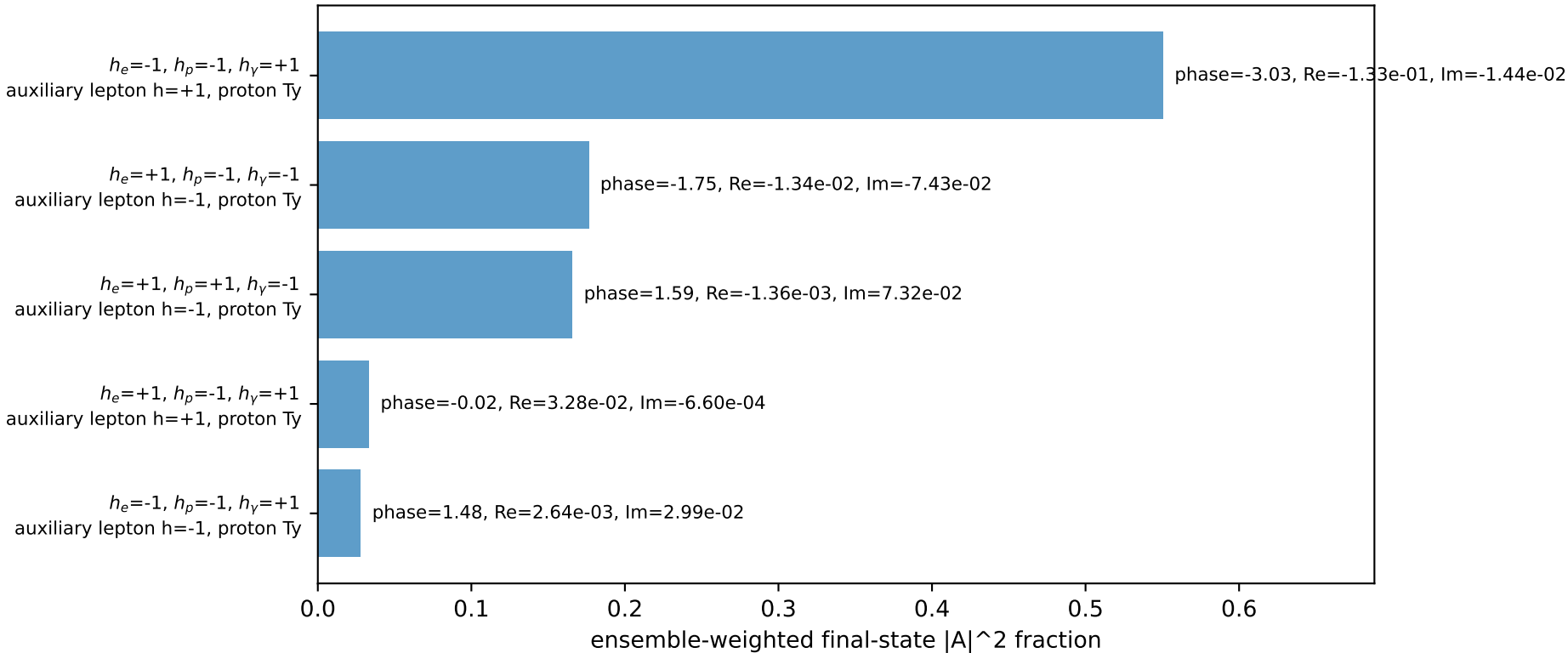
Leading initial-ensemble/final-state components (N=5, retained=95.4%)
