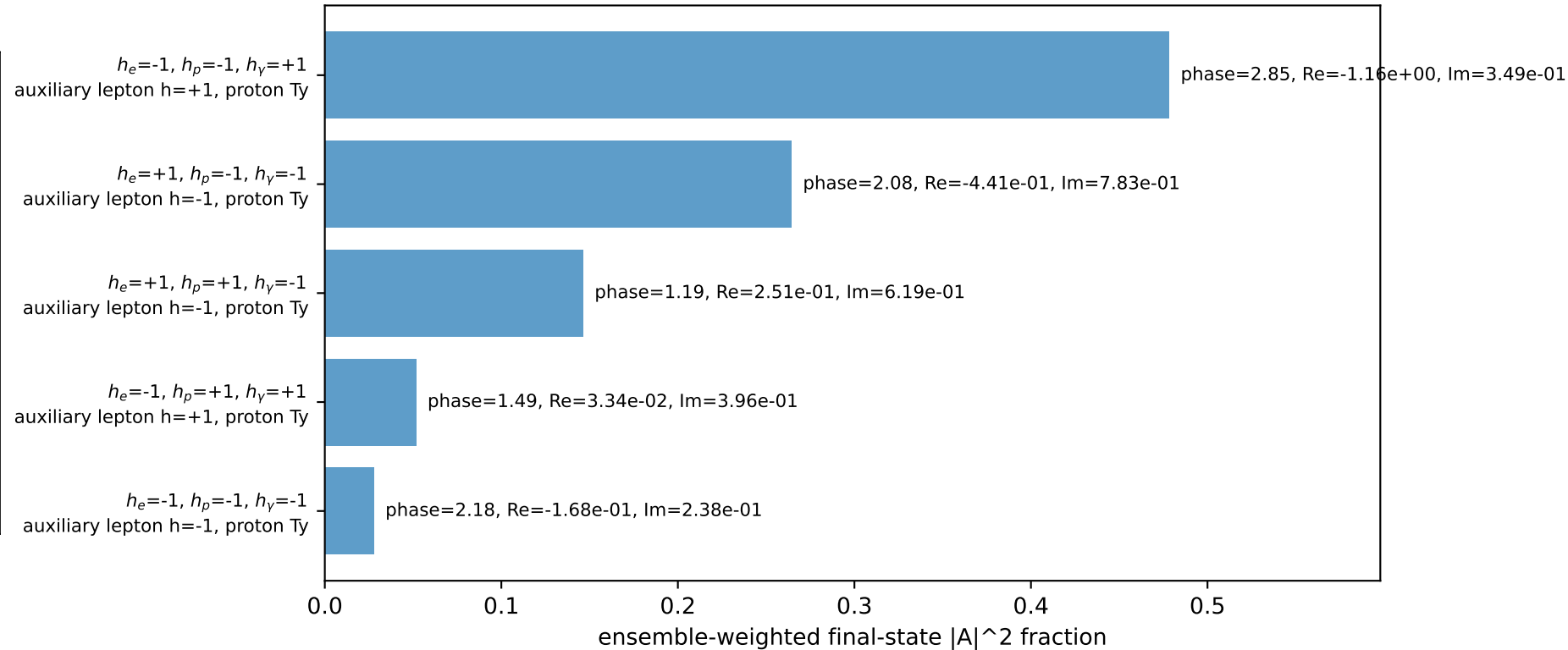
Leading initial-ensemble/final-state components (N=5, retained=96.8%)
