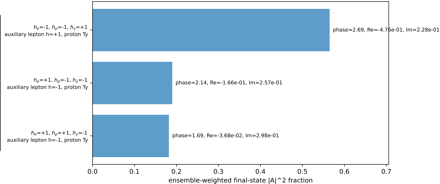
Leading initial-ensemble/final-state components (N=3, retained=93.7%)
