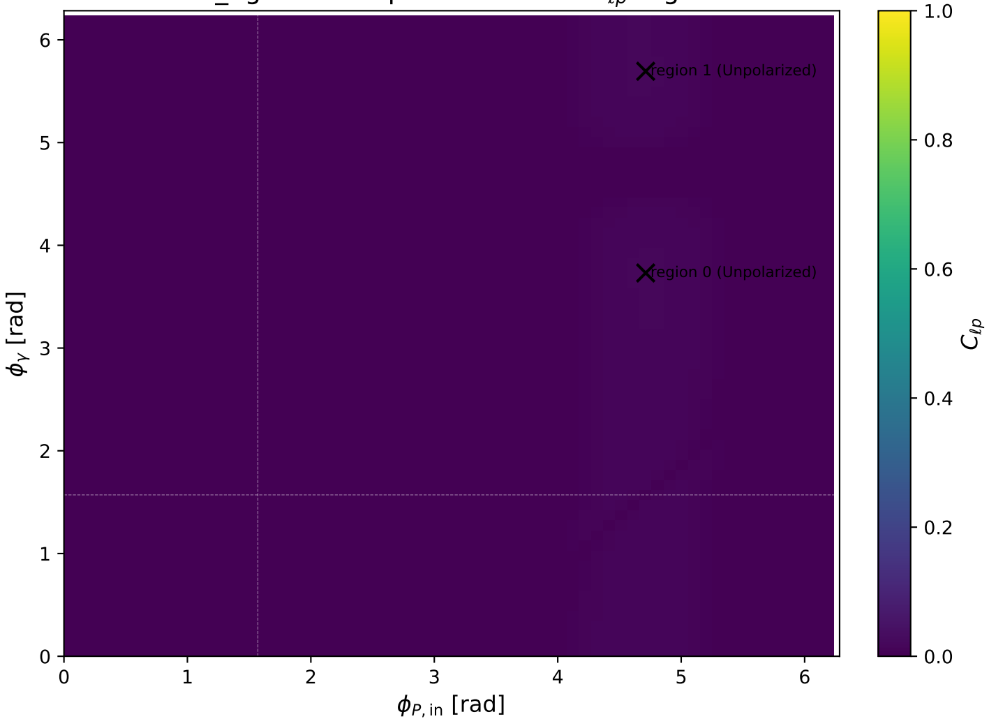
low_Egamma Unpolarized: max C_{lp} regions
