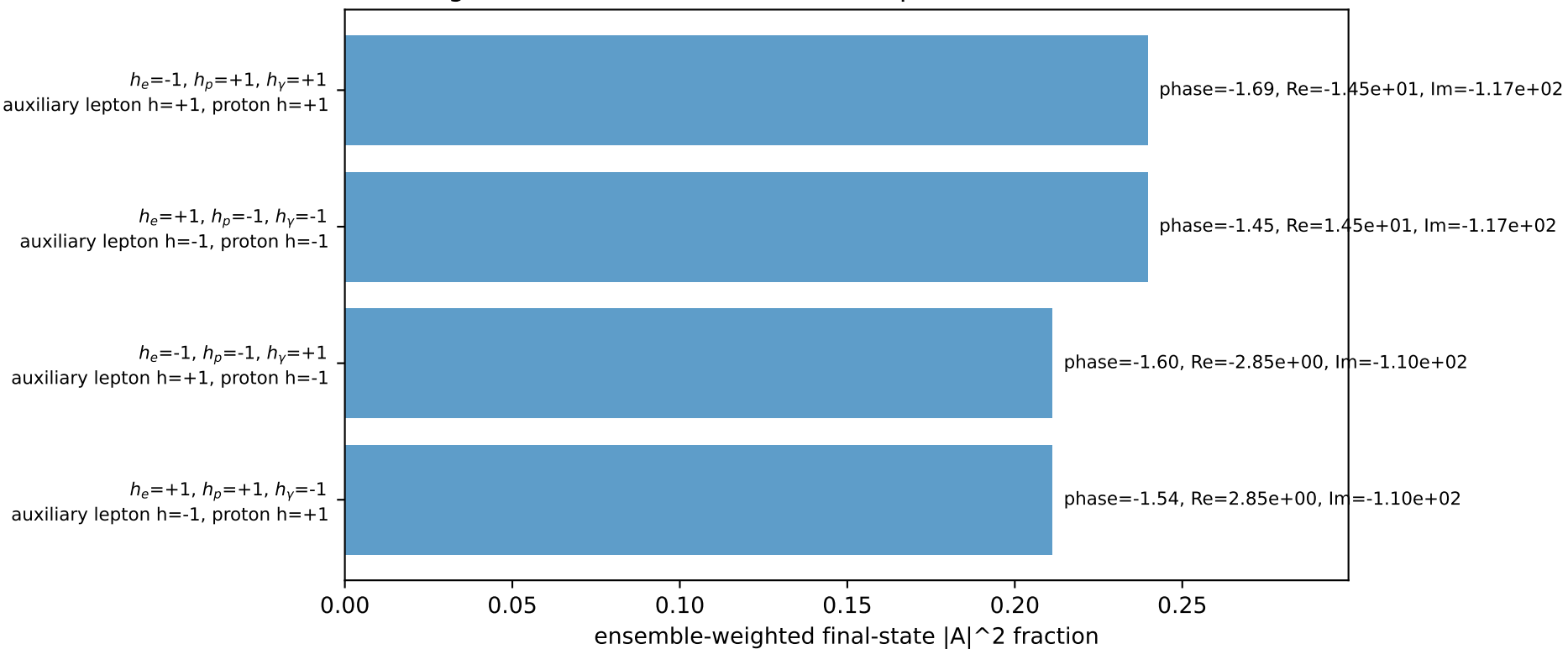
Leading initial-ensemble/final-state components (N=4, retained=90.2%)
