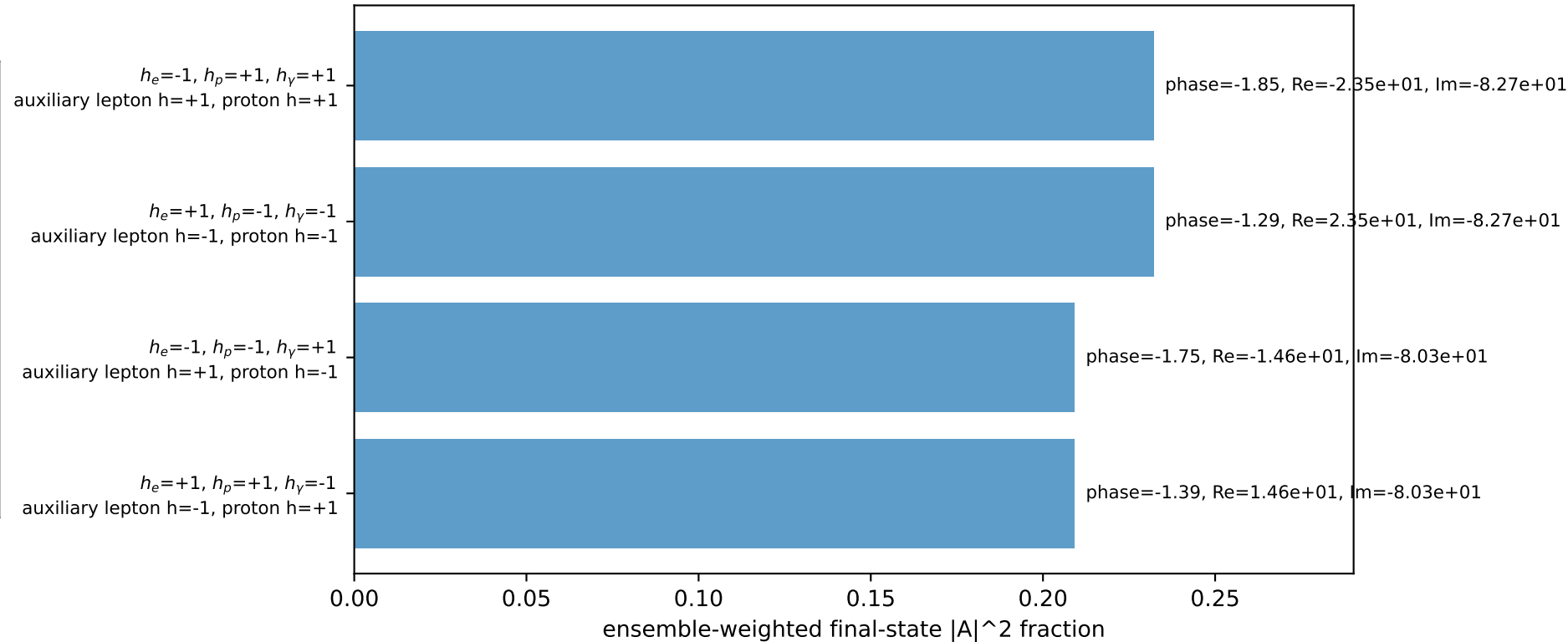
Leading initial-ensemble/final-state components (N=4, retained=88.3%)
