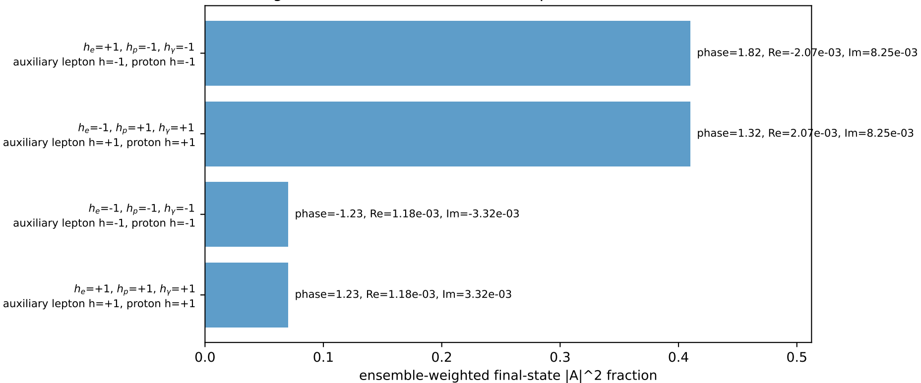
Leading initial-ensemble/final-state components (N=4, retained=96.0%)
