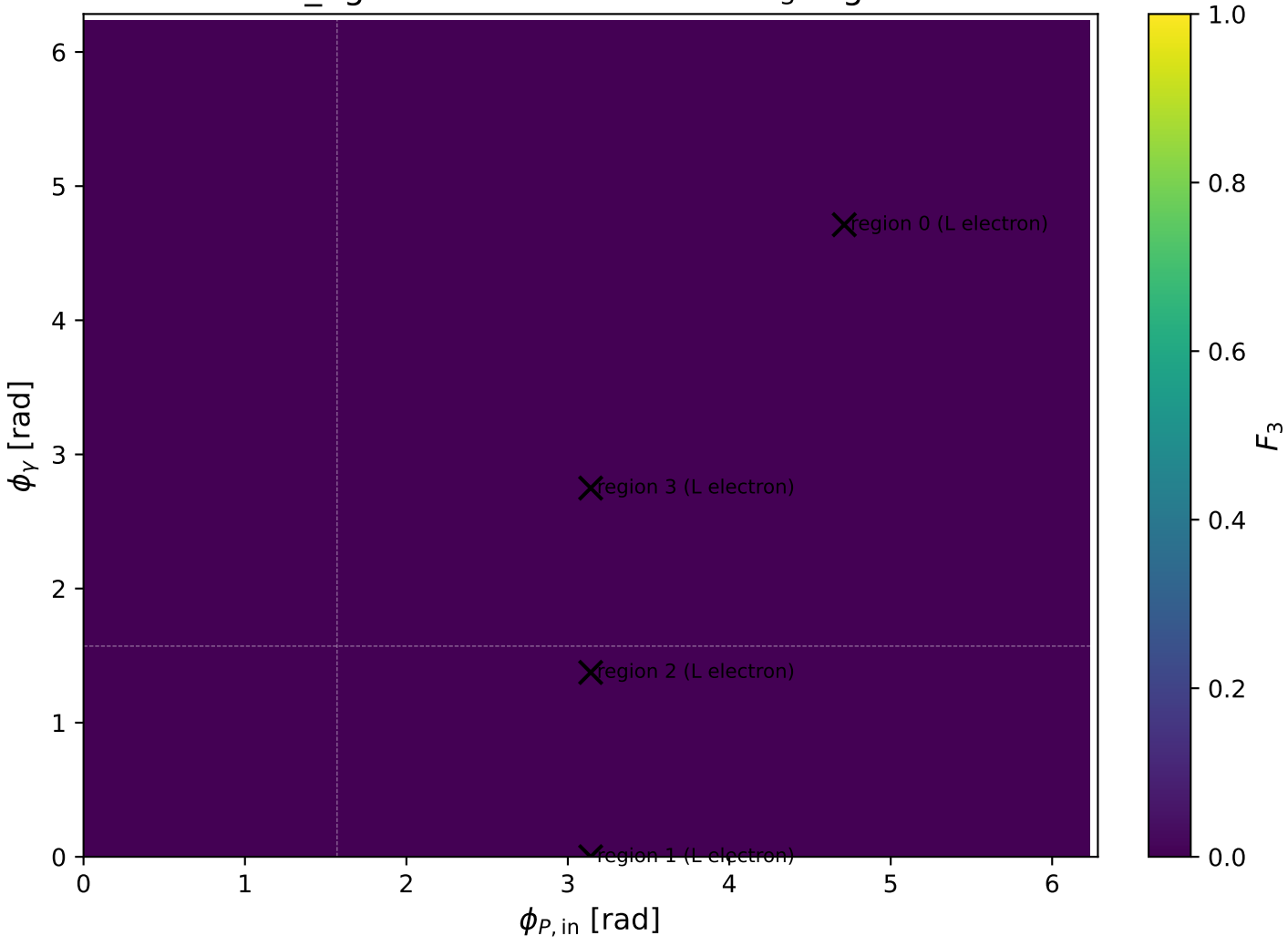
low_Egamma L electron: max F_3 regions
