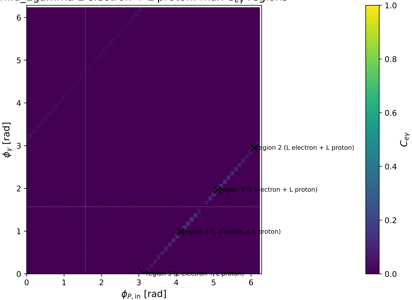
mid_Egamma L electron + L proton: max C_{e\gamma} regions
