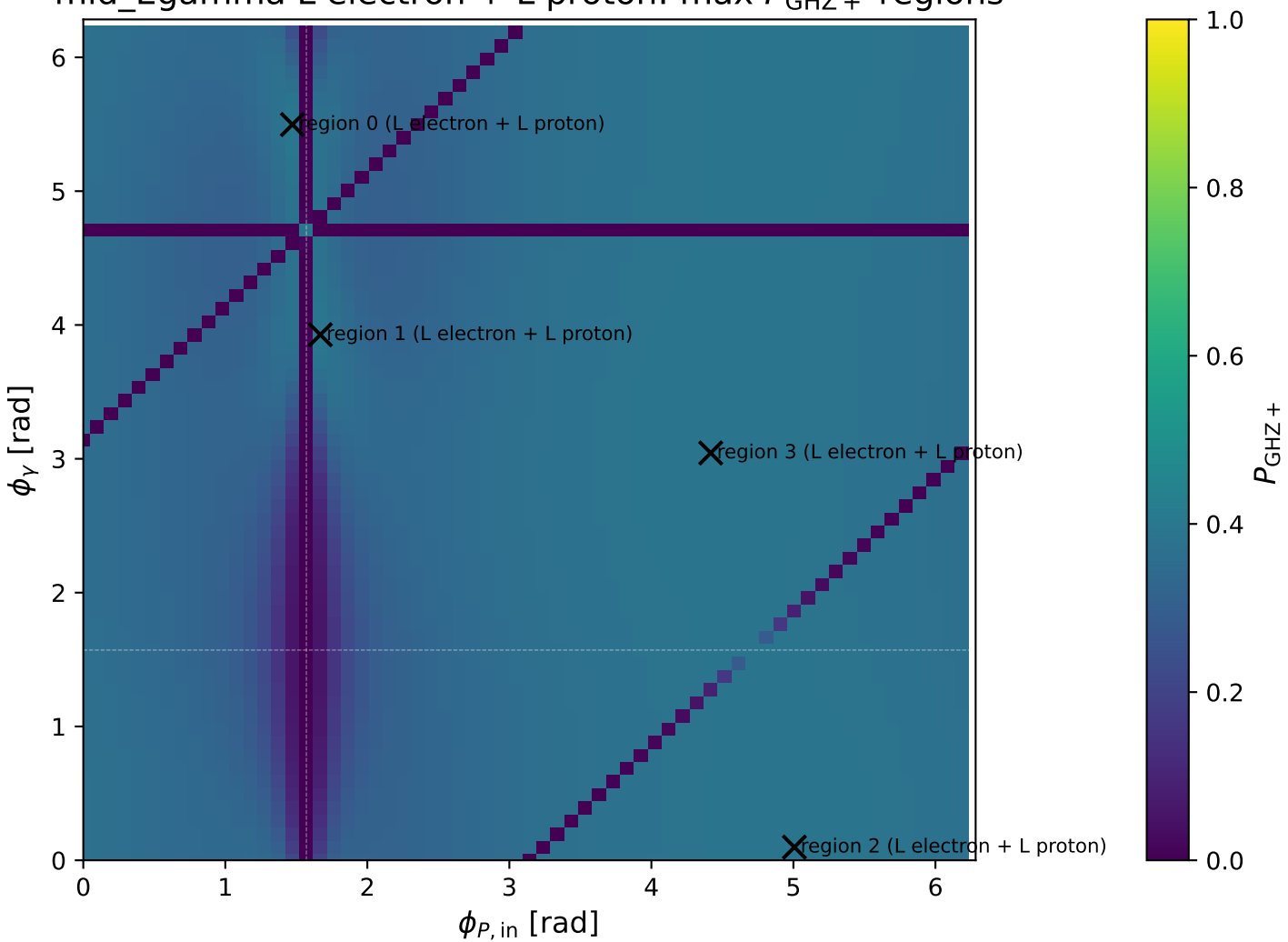
mid_Egamma L electron + L proton: max P_{\text{GHZ}+} regions
