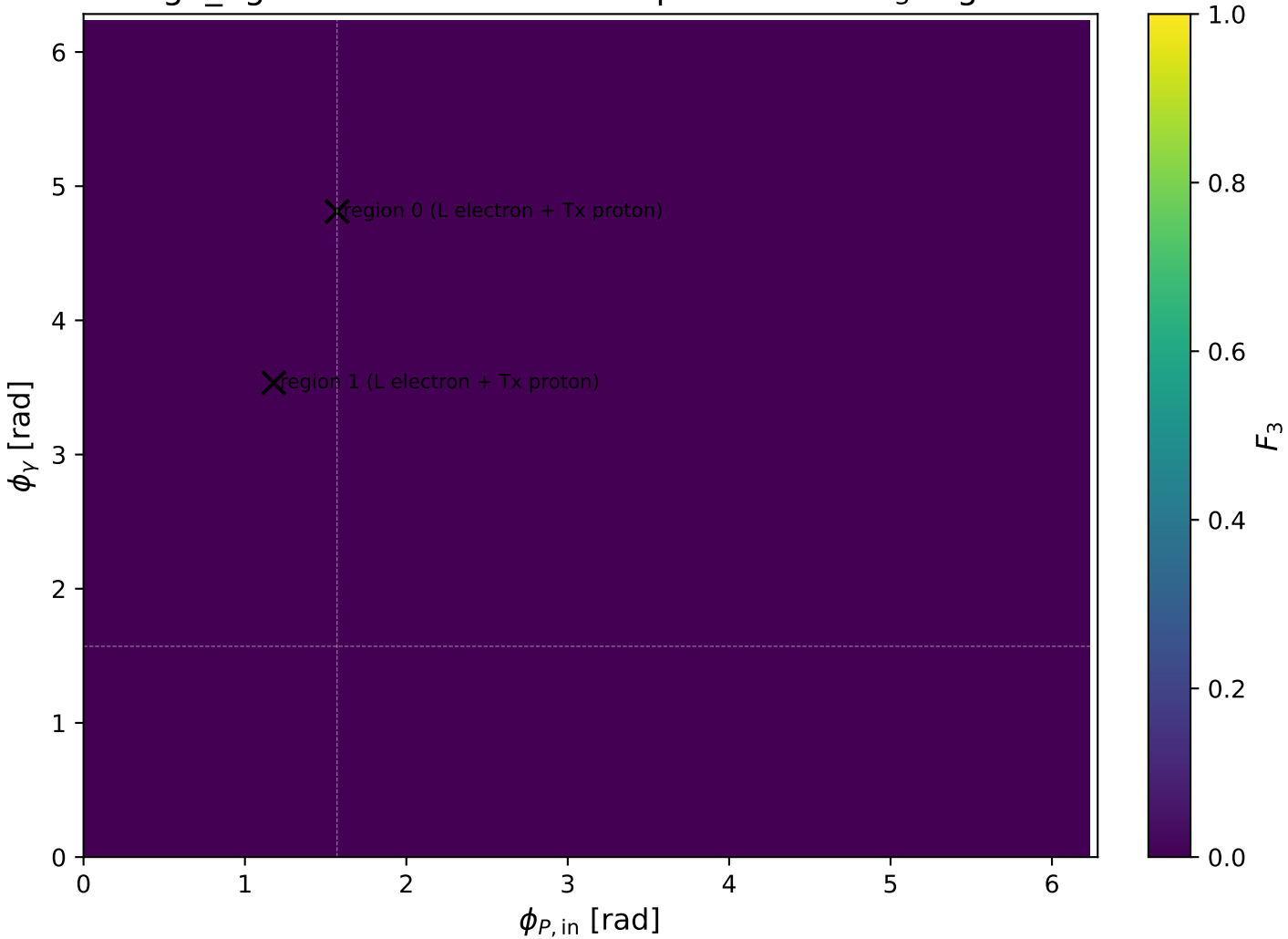
high_Egamma L electron + Tx proton: max F_3 regions
