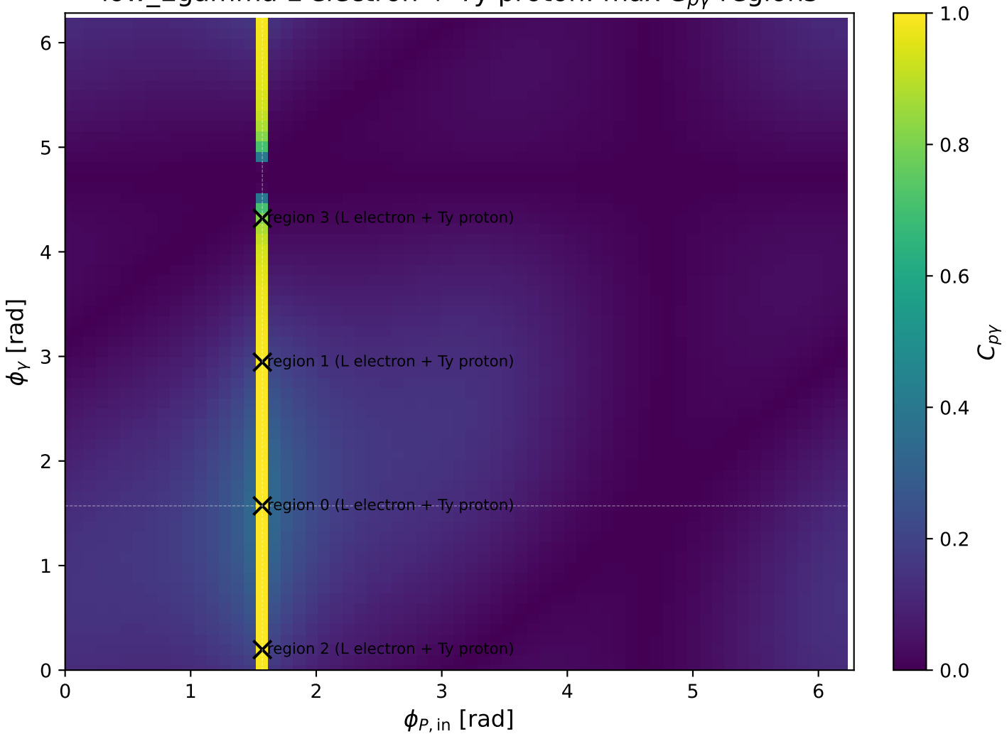
low_Egamma L electron + Ty proton: max C_{p\gamma} regions
