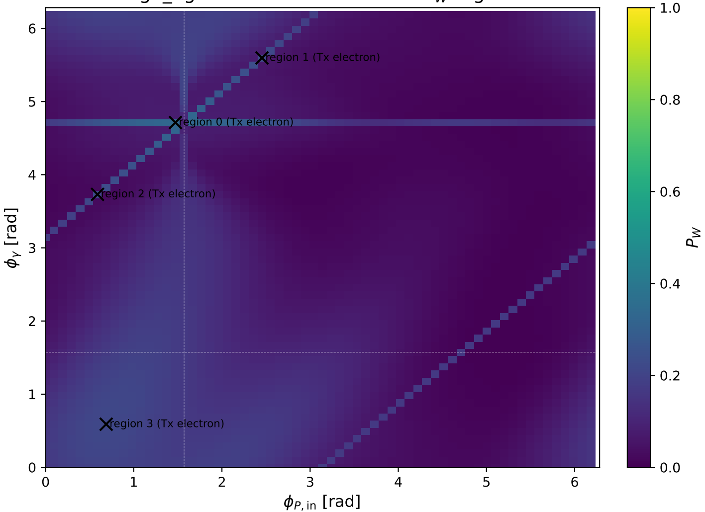
high_Egamma Tx electron: max P_W regions
