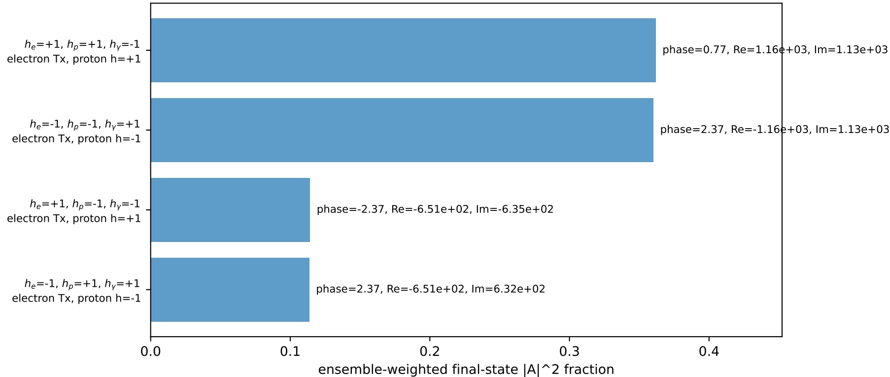
Leading initial-ensemble/final-state components (N=4, retained=95.0%)
