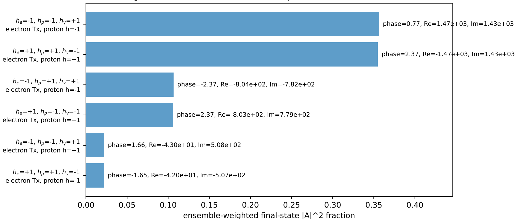
Leading initial-ensemble/final-state components (N=6, retained=96.7%)
