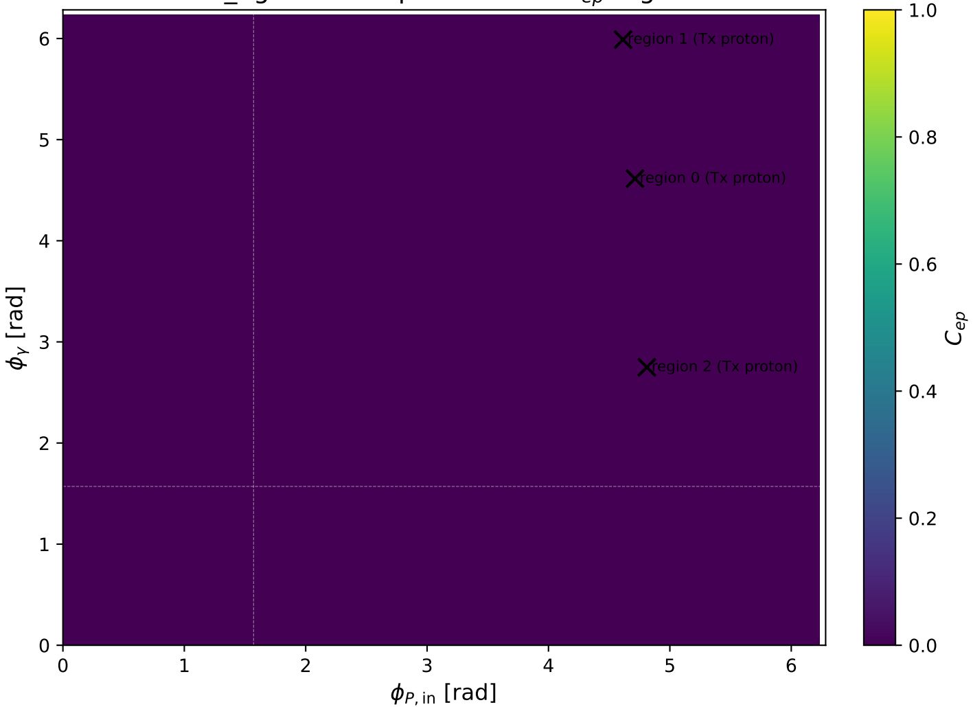
low_Egamma Tx proton: max C_{ep} regions
