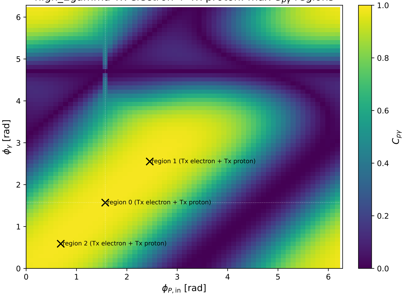
high_Egamma Tx electron + Tx proton: max C_{py} regions
