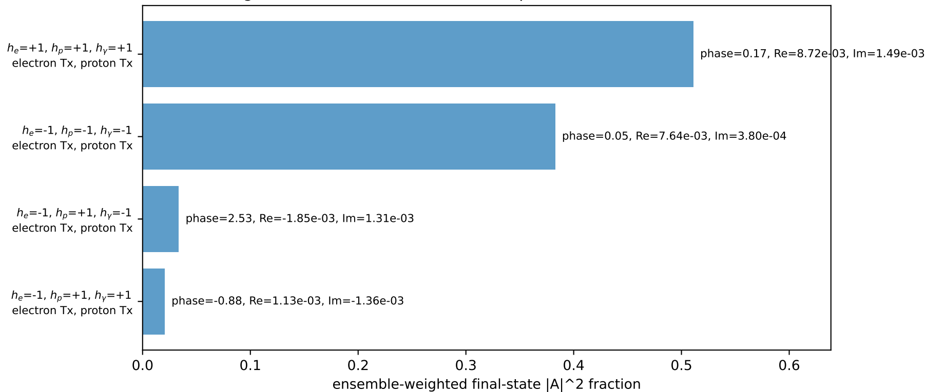
Leading initial-ensemble/final-state components (N=4, retained=94.8%)
