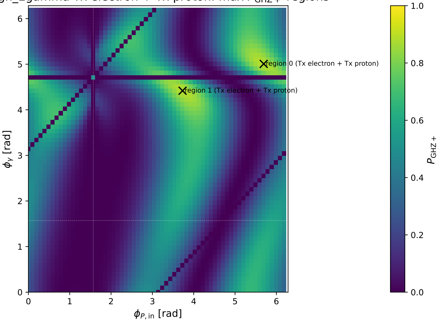
gh_Egamma Tx electron + Tx proton: max P_{\text{GHz}} + regions
