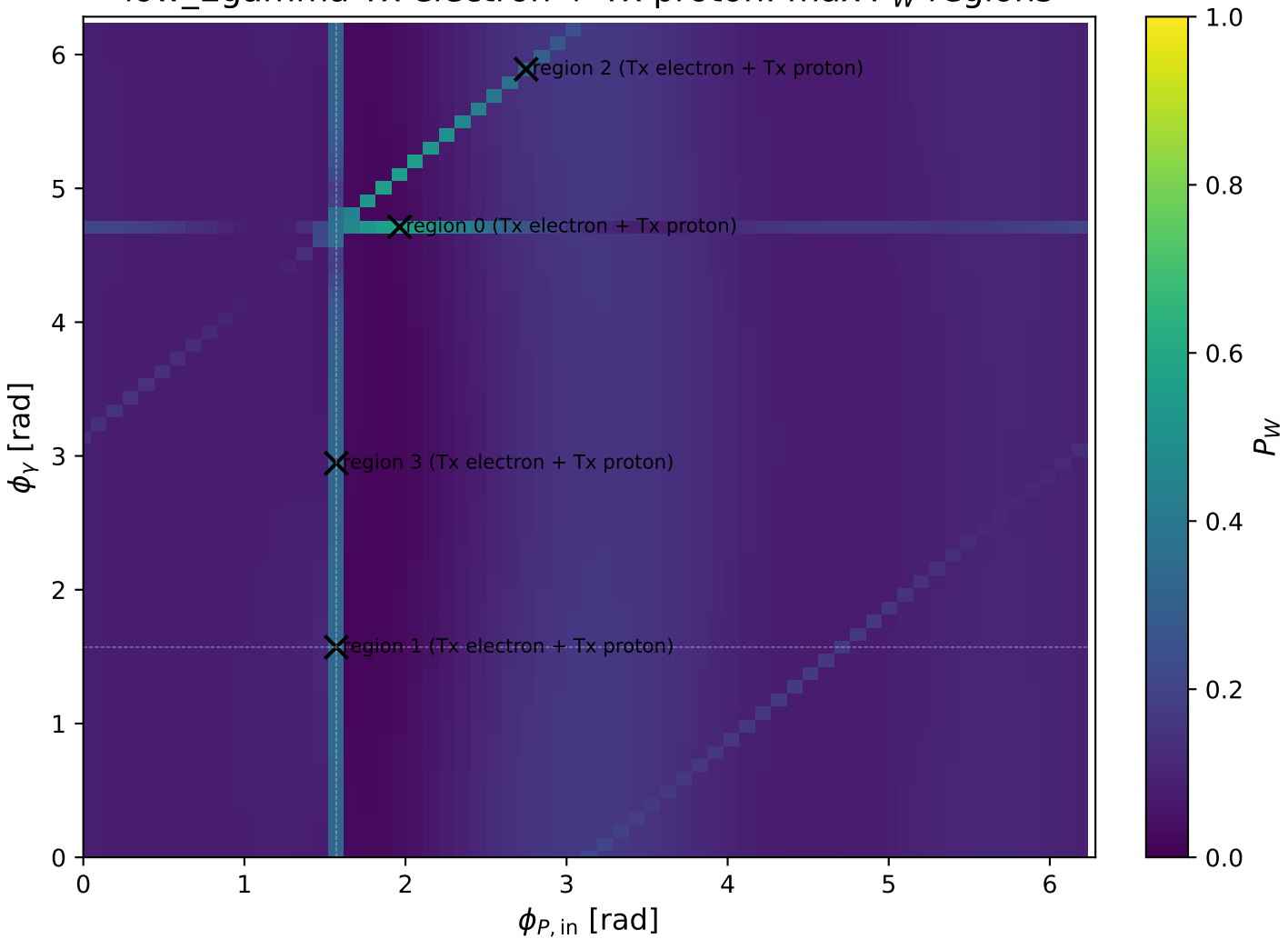
low_Egamma Tx electron + Tx proton: max P_W regions
