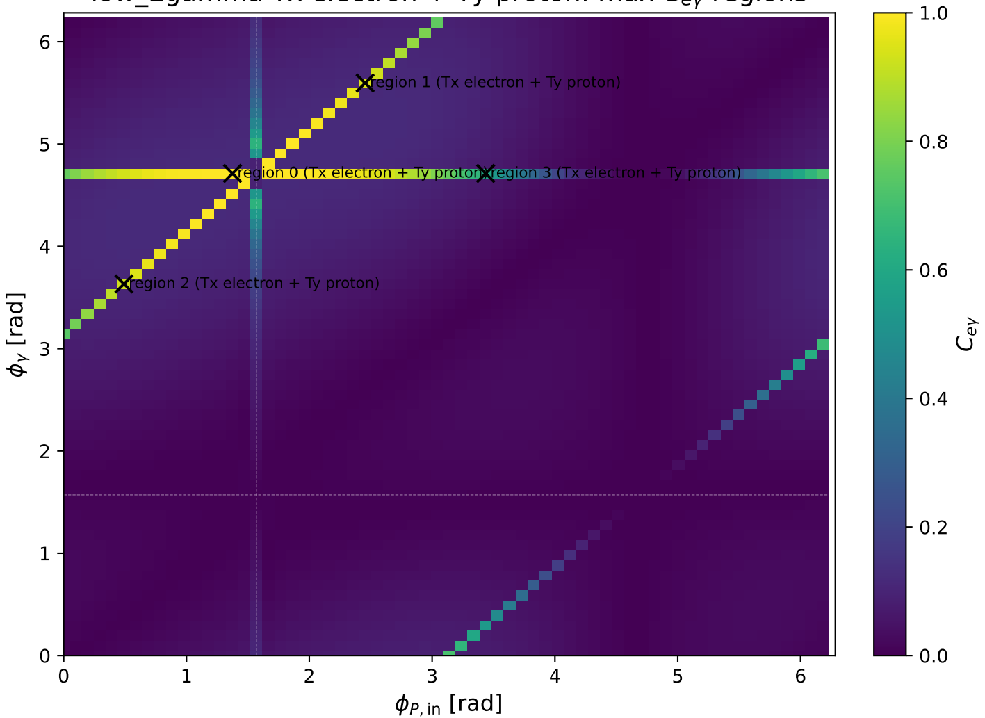
low_Egamma Tx electron + Ty proton: max C_{e\gamma} regions
