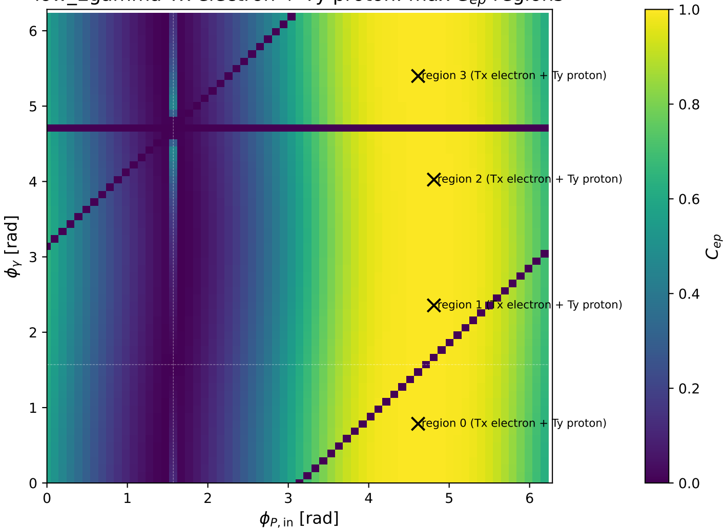
low_Egamma Tx electron + Ty proton: max C_{ep} regions
