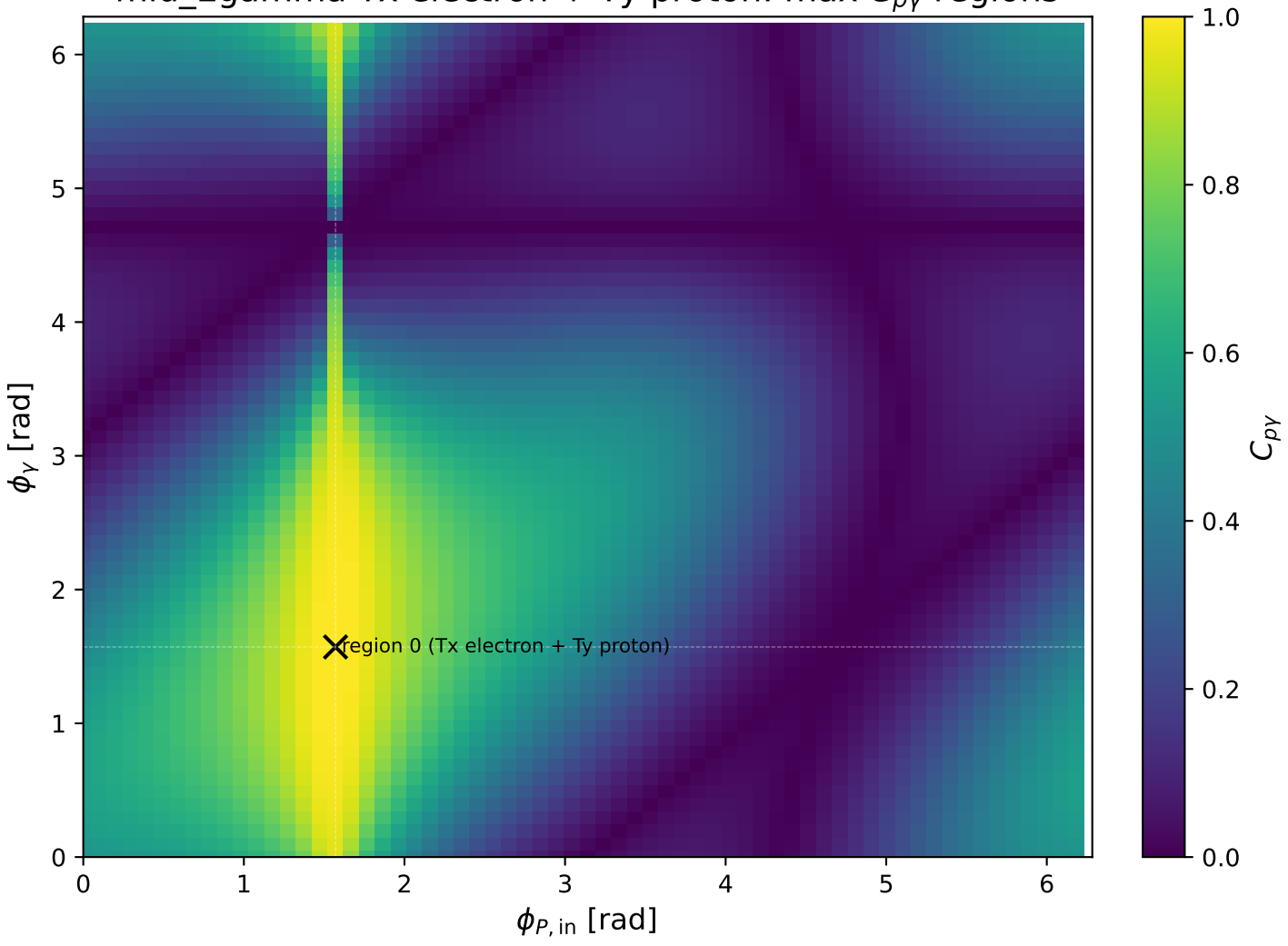
mid_Egamma Tx electron + Ty proton: max C_{p\gamma} regions
