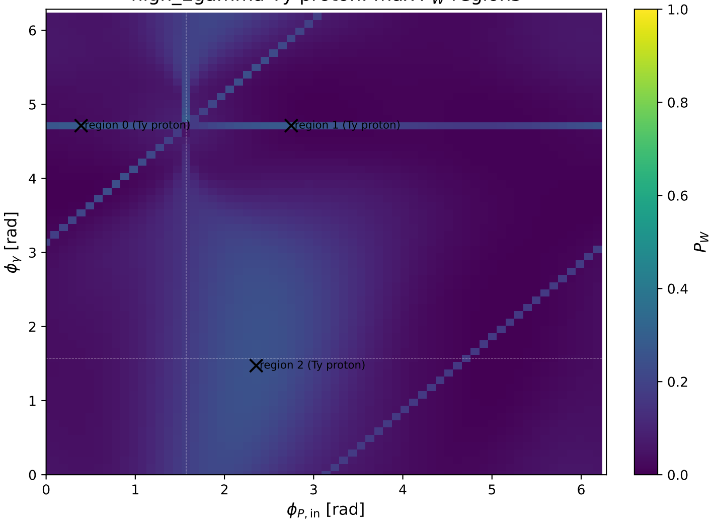
high_Egamma Ty proton: max P_W regions
