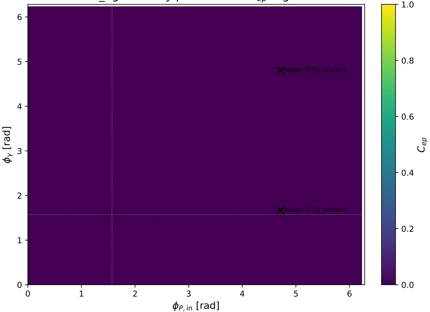
low_Egamma Ty proton: max C_{ep} regions
