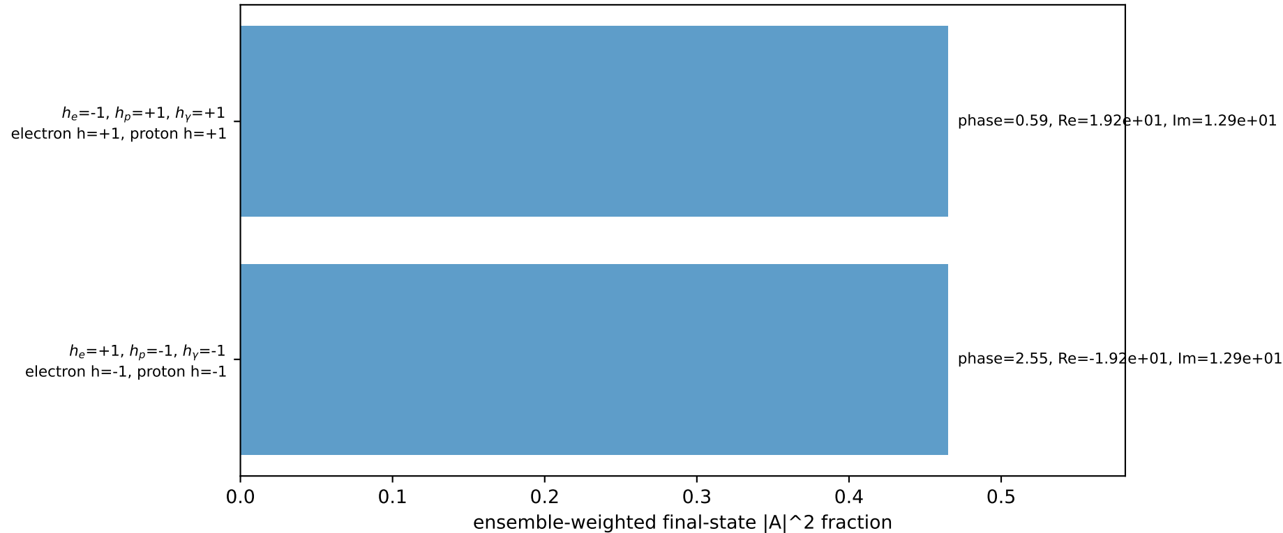
Leading initial-ensemble/final-state components (N=2, retained=93.1%)
