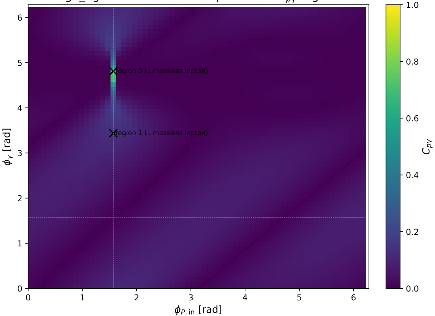
high_Egamma L massless lepton: max C_{p\gamma} regions
