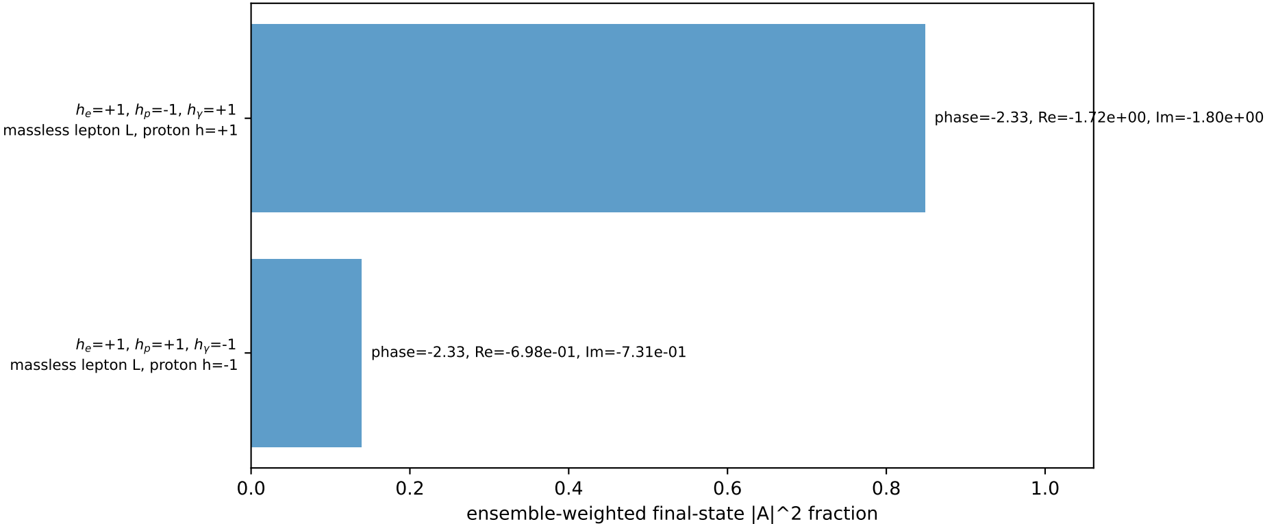
Leading initial-ensemble/final-state components (N=2, retained=98.8%)
