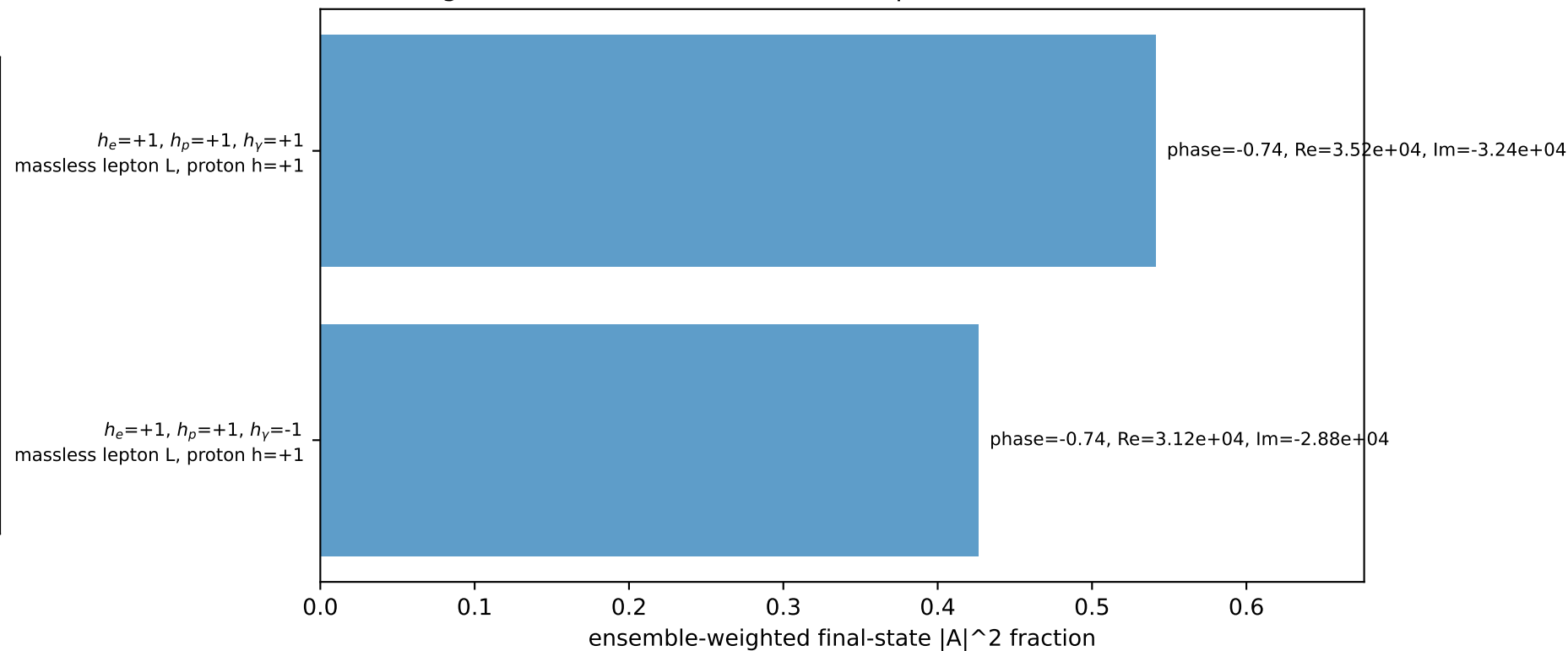
Leading initial-ensemble/final-state components (N=2, retained=96.7%)
