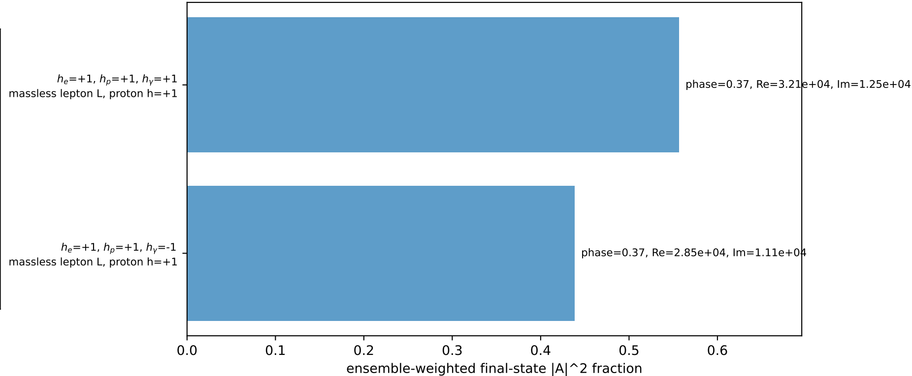
Leading initial-ensemble/final-state components (N=2, retained=99.5%)
