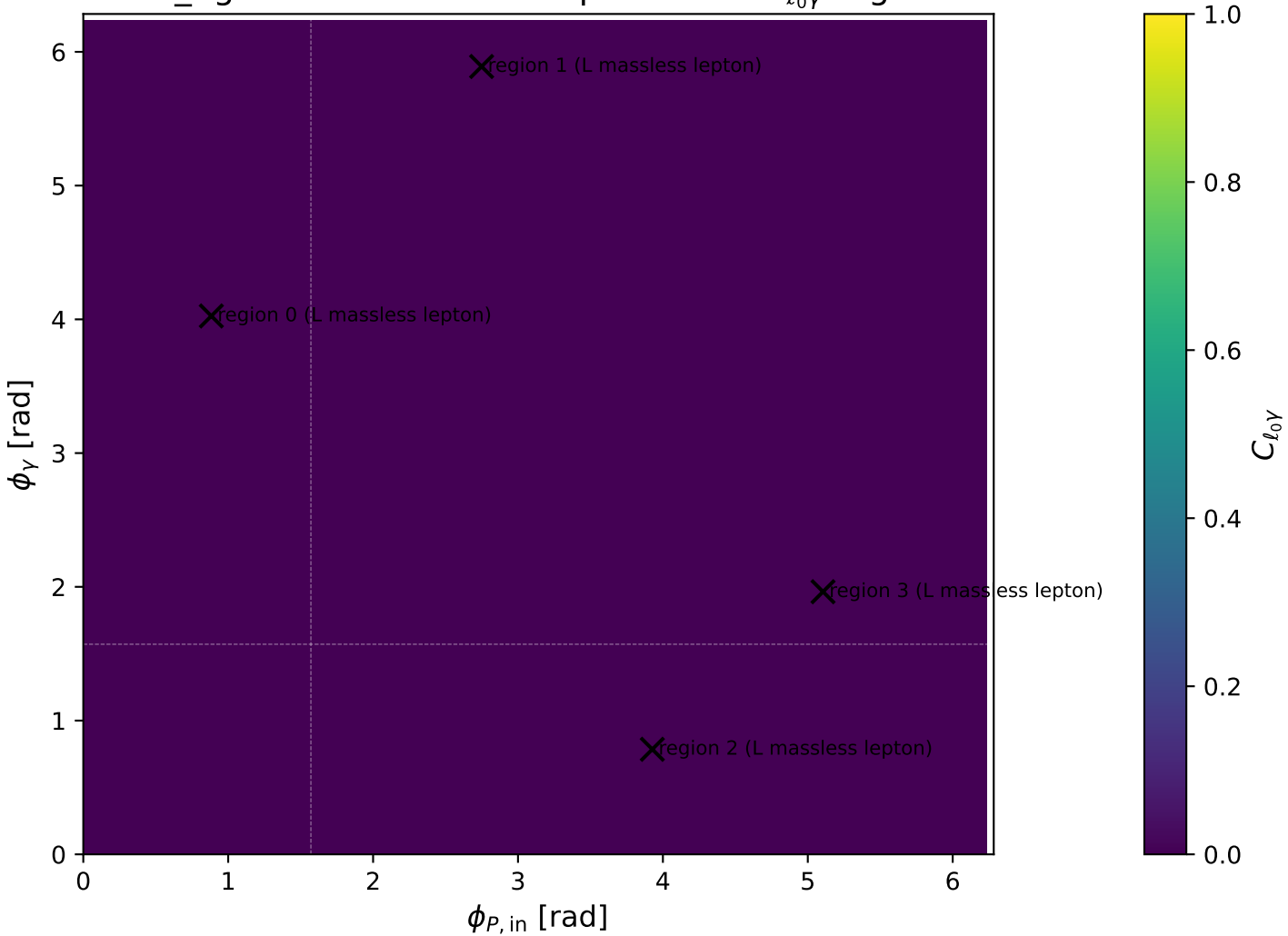
low_Egamma L massless lepton: max C_{\ell_0\gamma} regions
