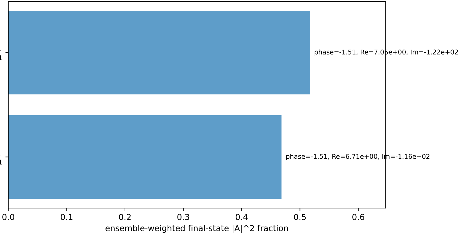
Leading initial-ensemble/final-state components (N=2, retained=98.6%)
