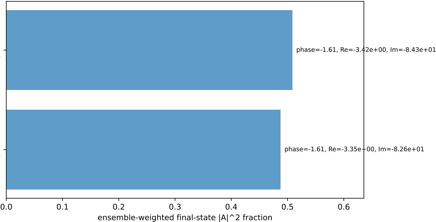
Leading initial-ensemble/final-state components (N=2, retained=99.6%)
