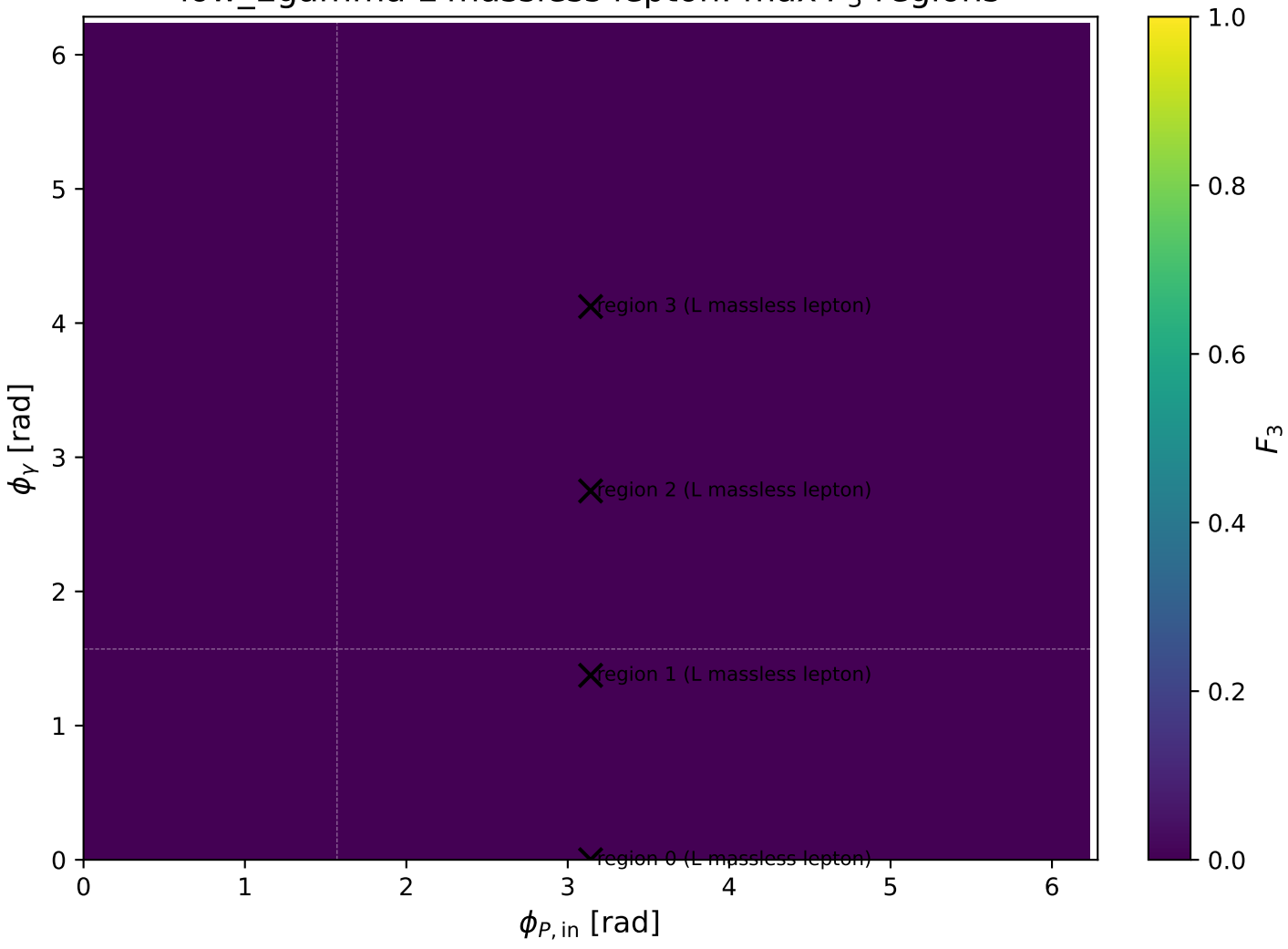
low_Egamma L massless lepton: max F_3 regions
