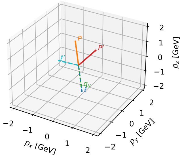
3D momenta
