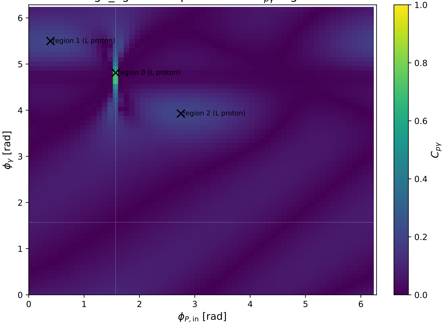
high_Egamma L proton: max C_{p\gamma} regions
