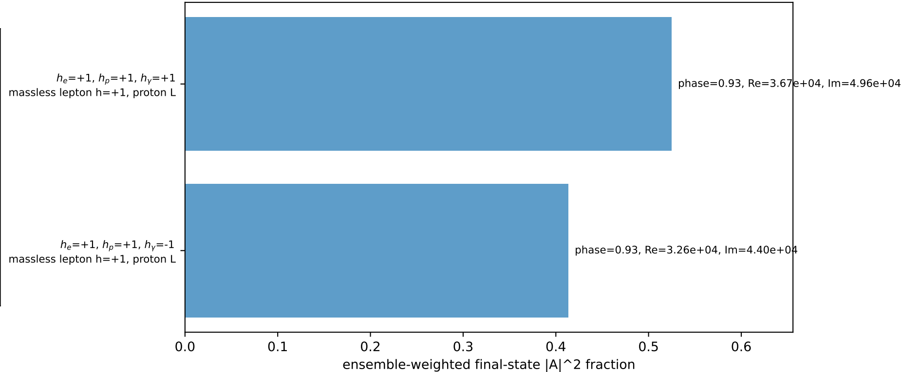
Leading initial-ensemble/final-state components (N=2, retained=93.8%)
