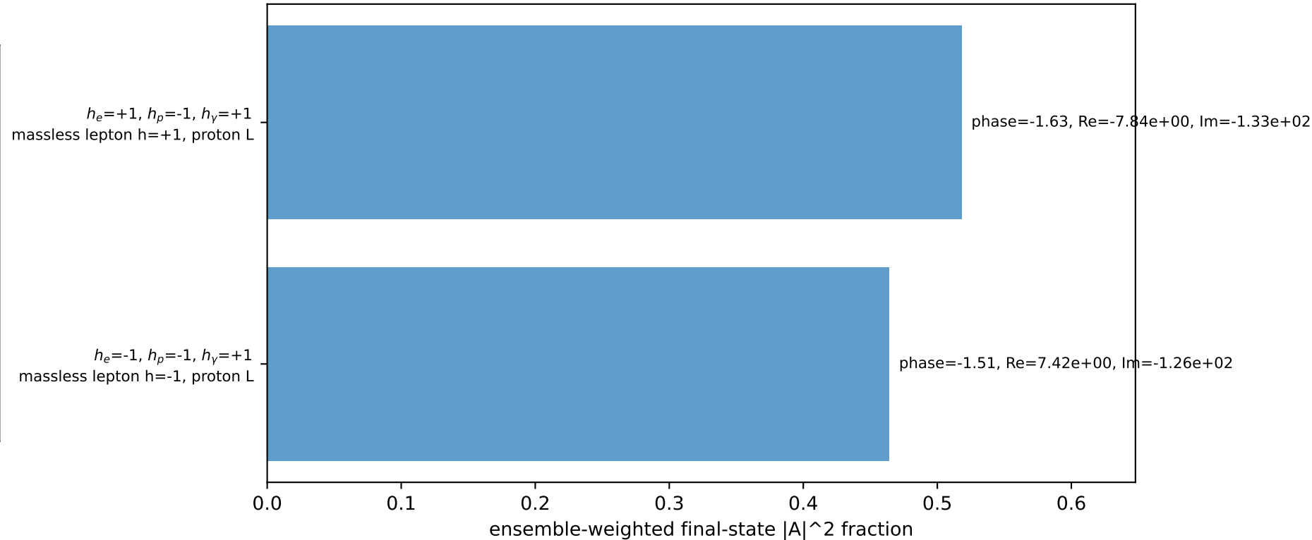
Leading initial-ensemble/final-state components (N=2, retained=98.3%)
