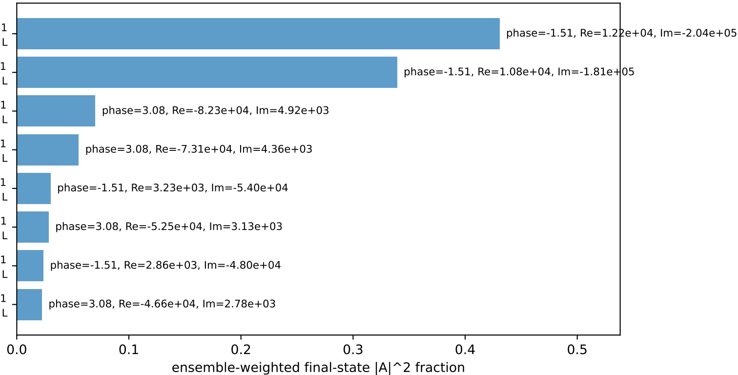
Leading initial-ensemble/final-state components (N=8, retained=100.0%)
