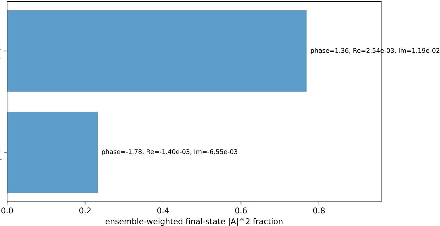
Leading initial-ensemble/final-state components (N=2, retained=99.9%)
