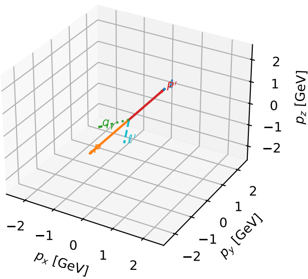
3D momenta
