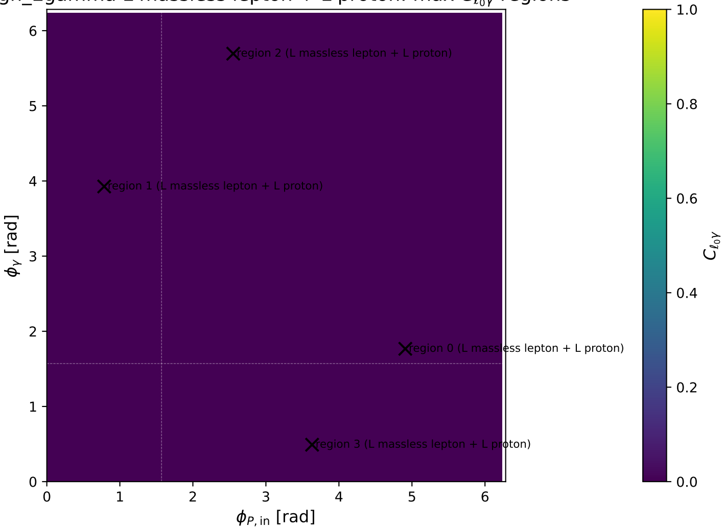
gh_Egamma L massless lepton + L proton: max C_{\ell_0\gamma} regions
