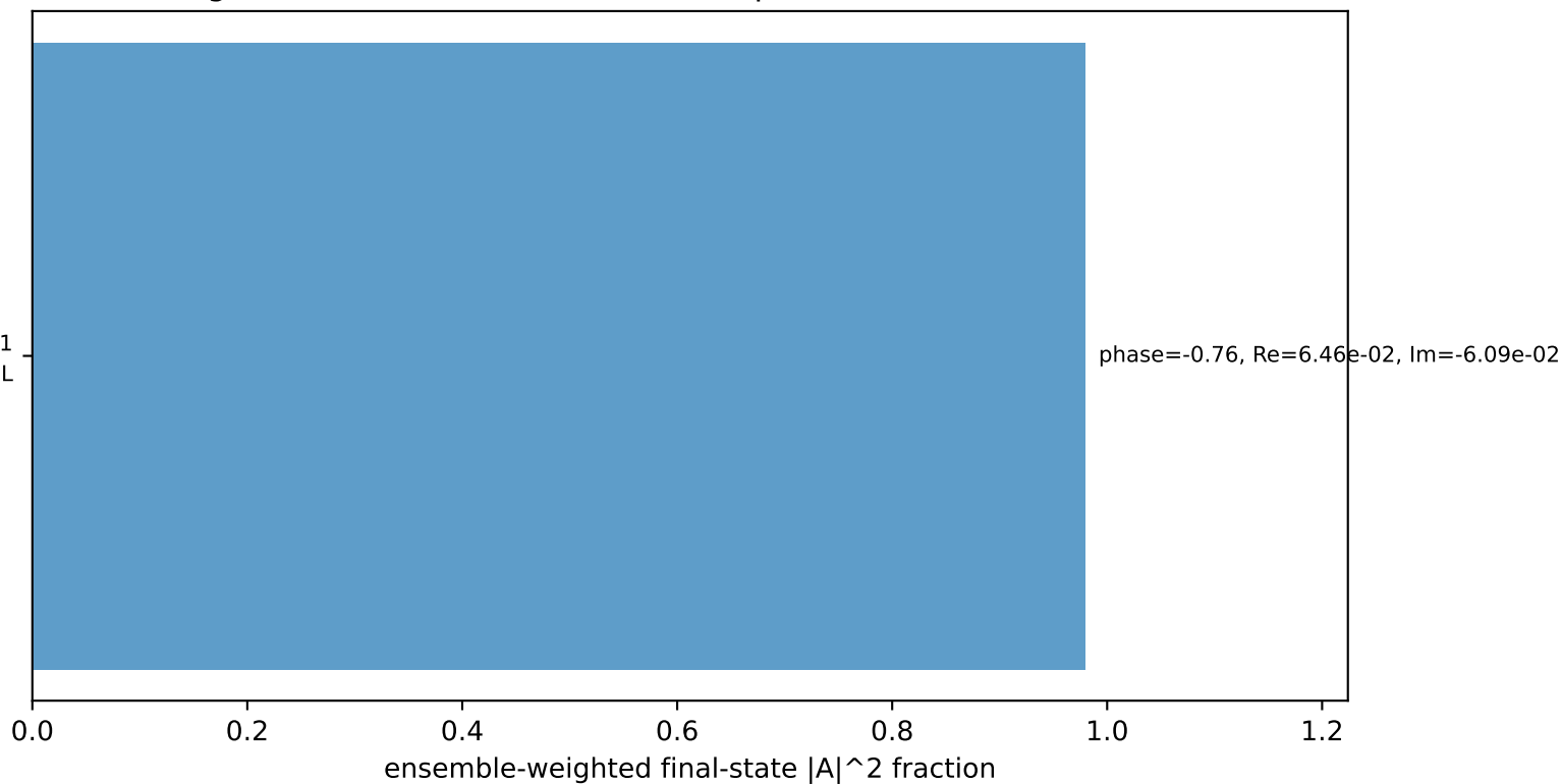
Leading initial-ensemble/final-state components (N=1, retained=97.9%)
