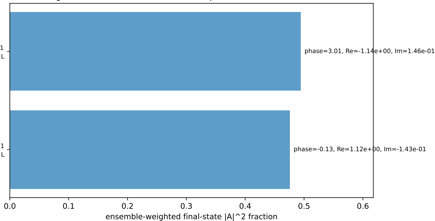
Leading initial-ensemble/final-state components (N=2, retained=97.0%)
