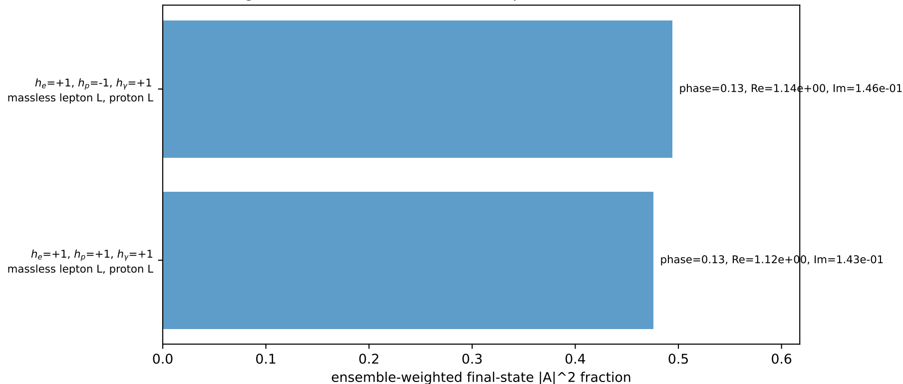
Leading initial-ensemble/final-state components (N=2, retained=97.0%)
