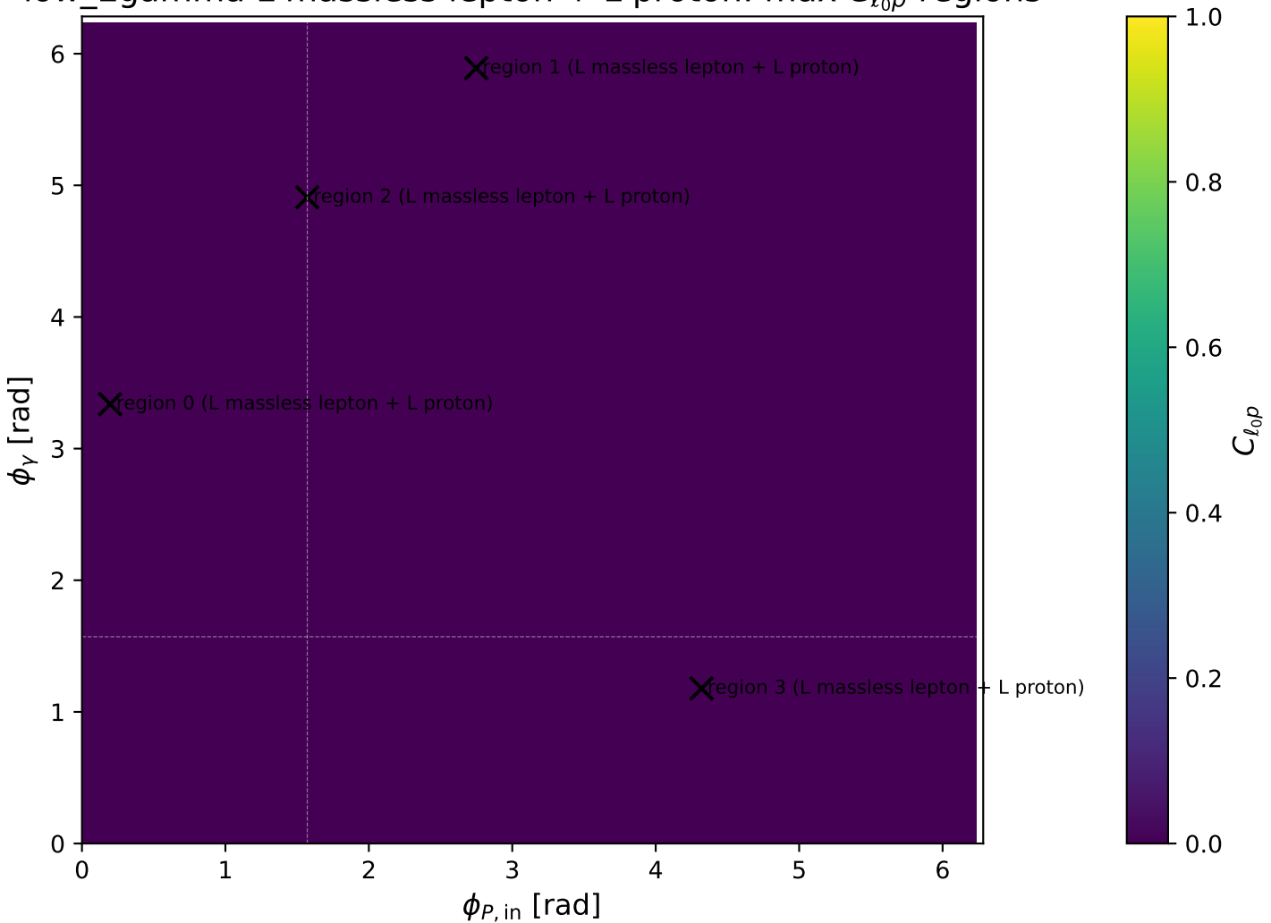
low_Egamma L massless lepton + L proton: max C_{\ell_0 p} regions
