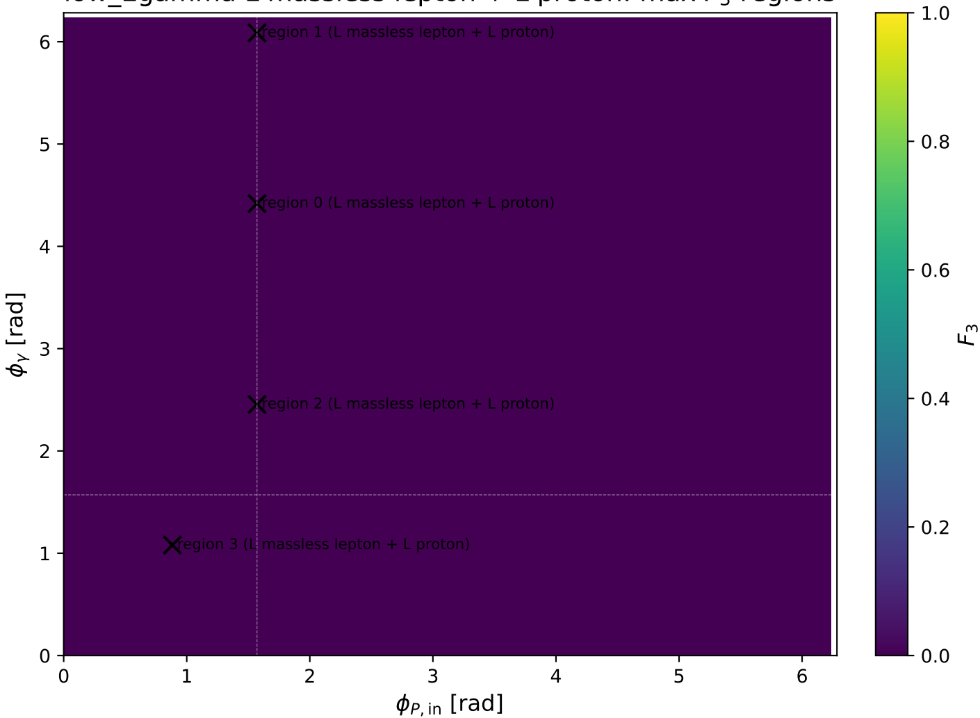
low_Egamma L massless lepton + L proton: max F_3 regions
