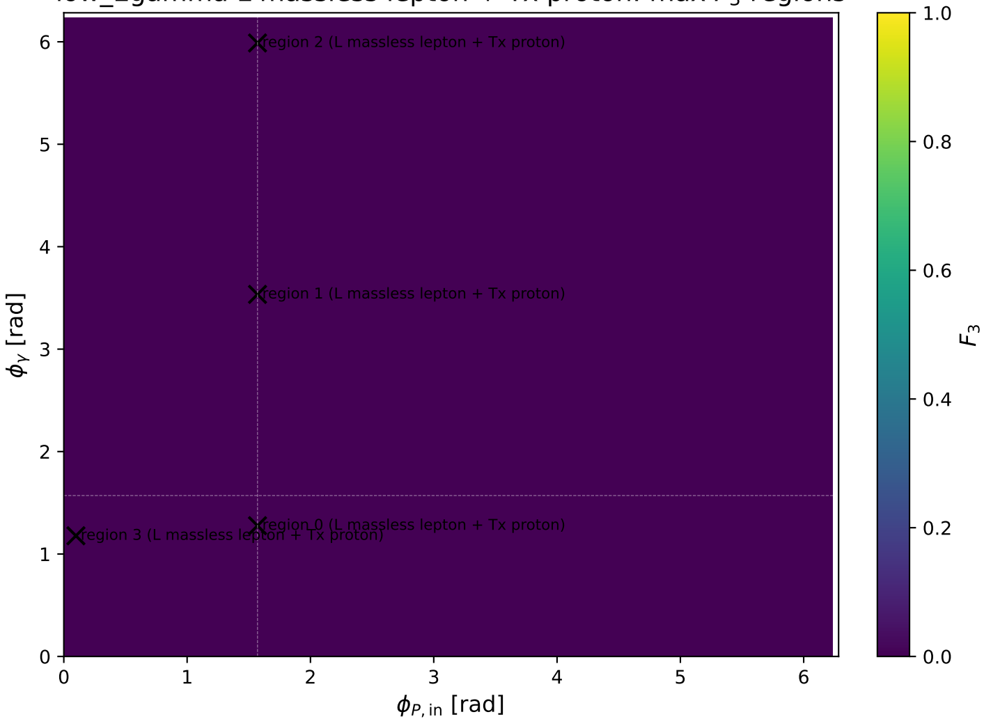
low_Egamma L massless lepton + Tx proton: max F_3 regions
