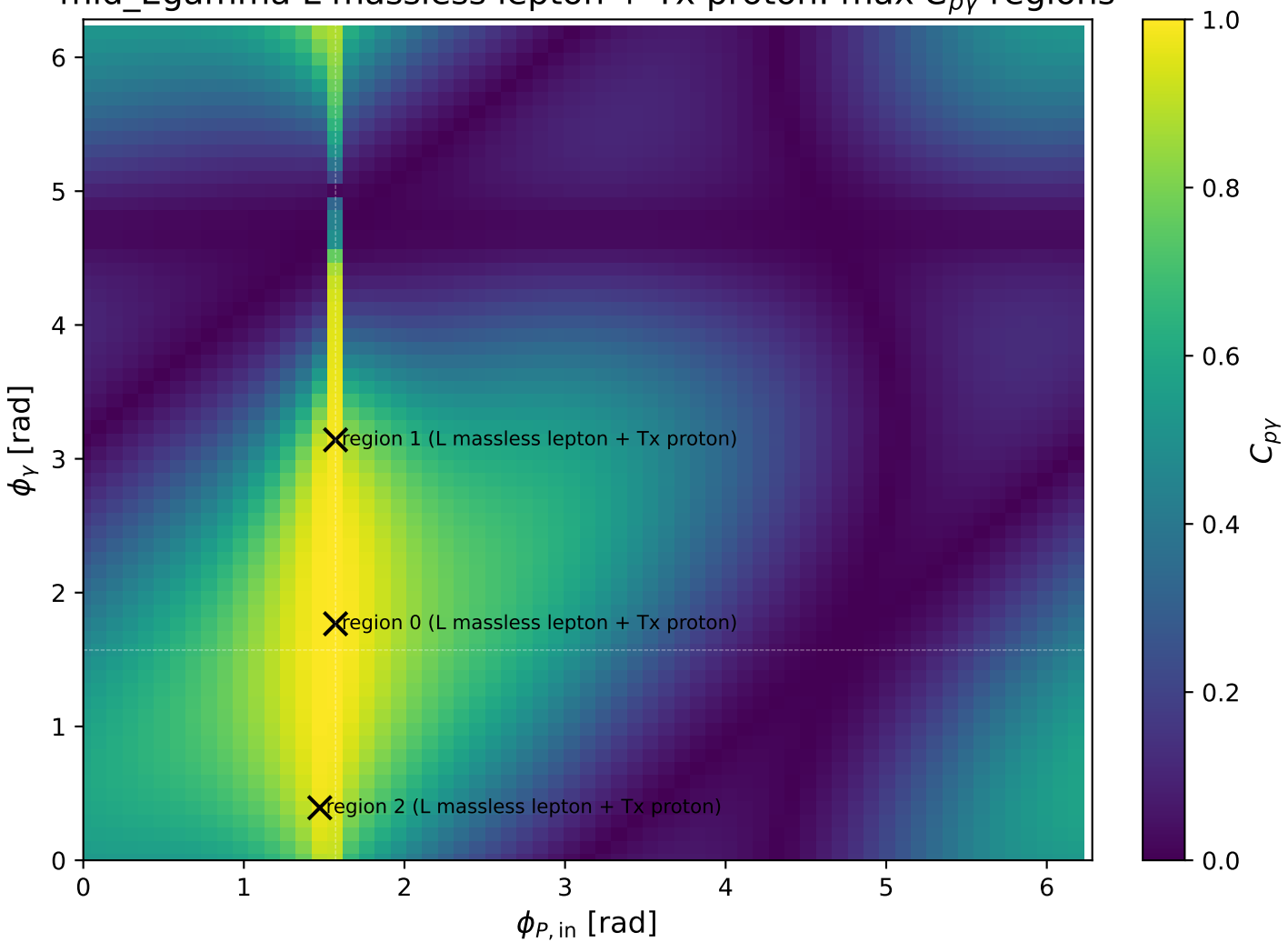
mid_Egamma L massless lepton + Tx proton: max C_{p\gamma} regions
