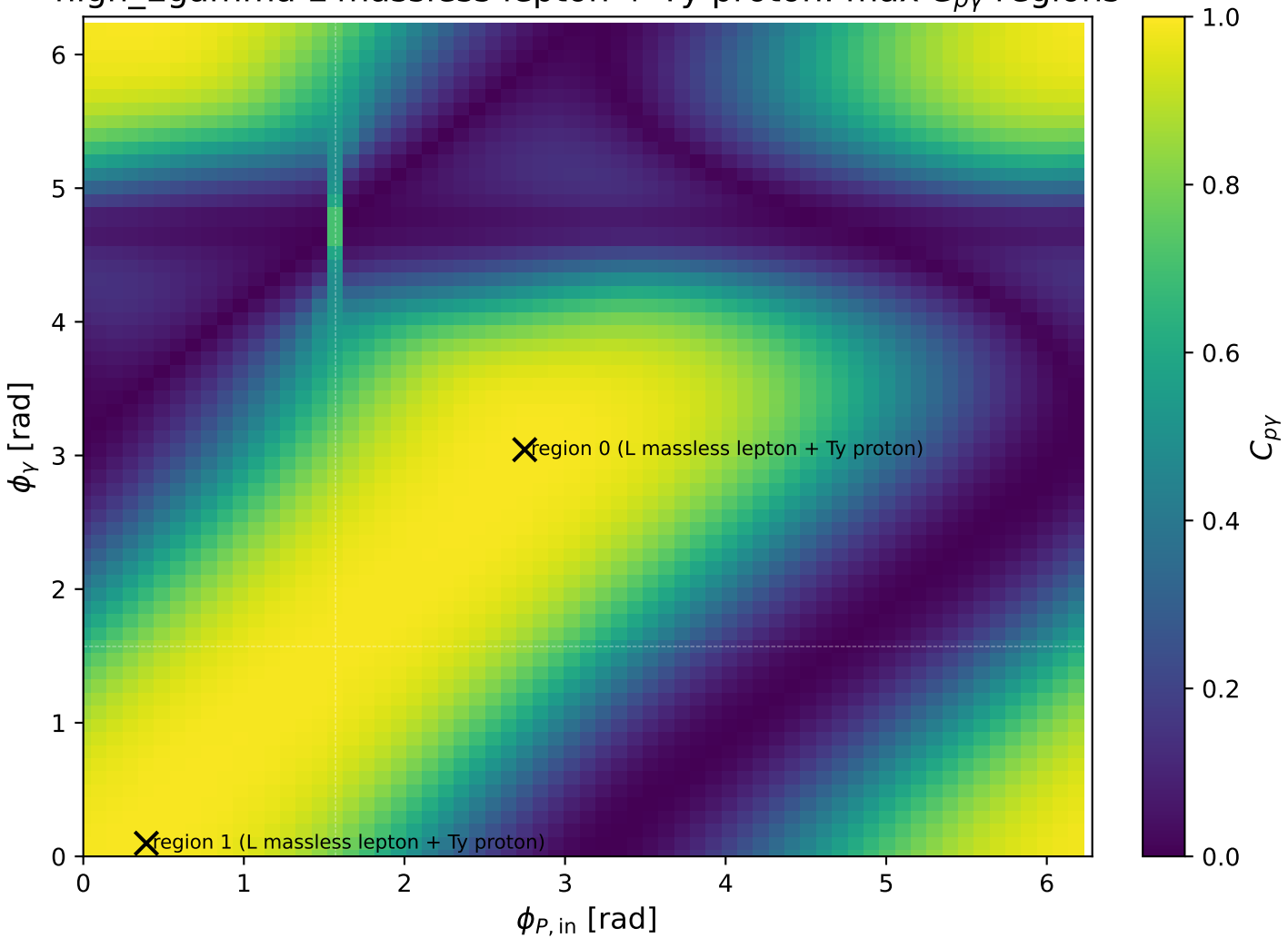
high_Egamma L massless lepton + Ty proton: max C_{p\gamma} regions
