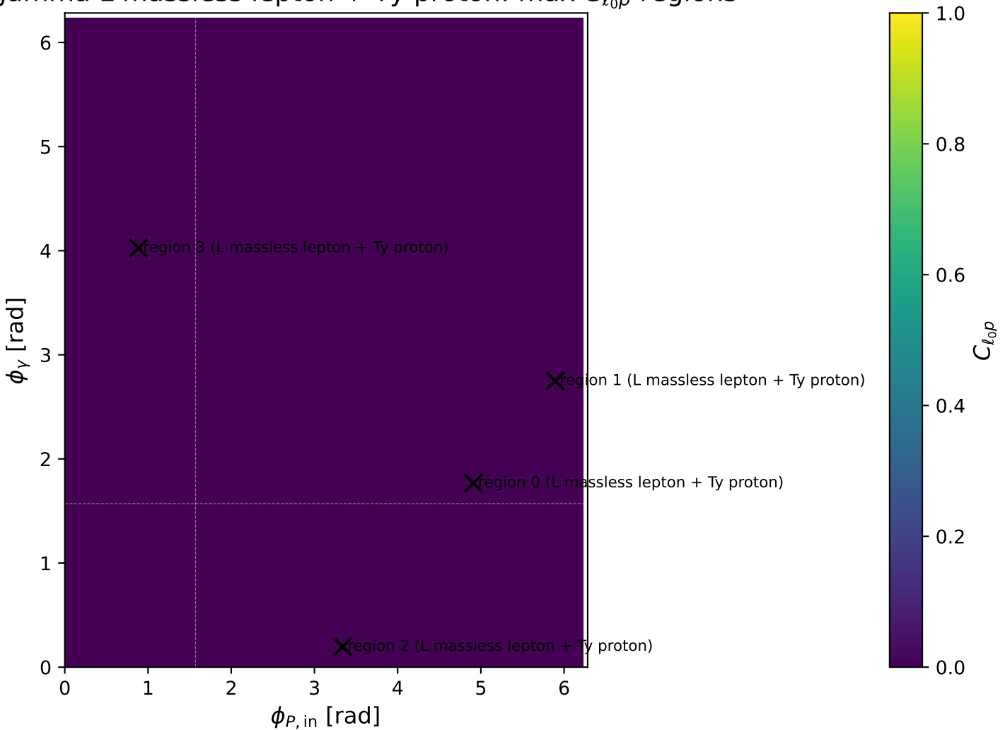
gamma L massless lepton + Ty proton: max C_{\ell_0 p} regions
