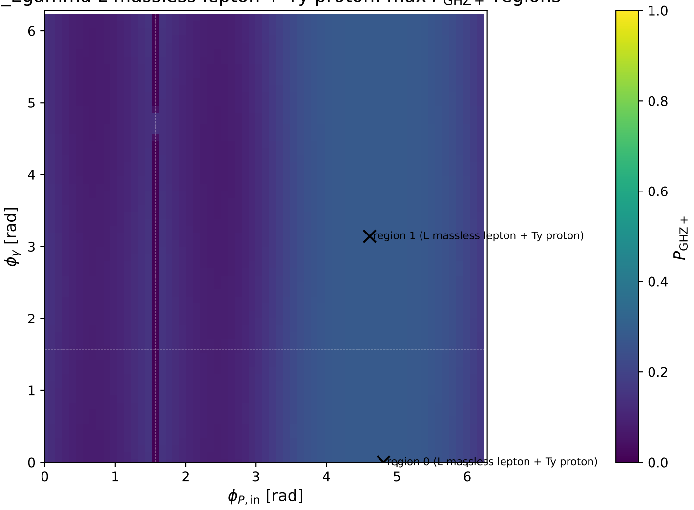
\gamma L massless lepton + Ty proton: max P_{\text{GHZ}} regions
