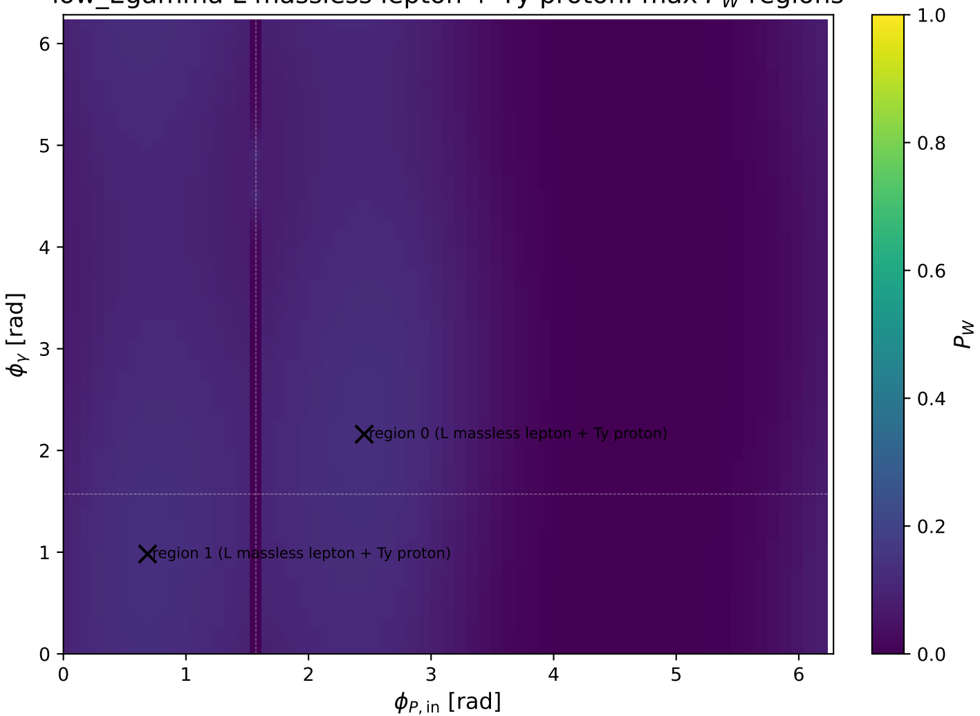
low_Egamma L massless lepton + Ty proton: max P_W regions
