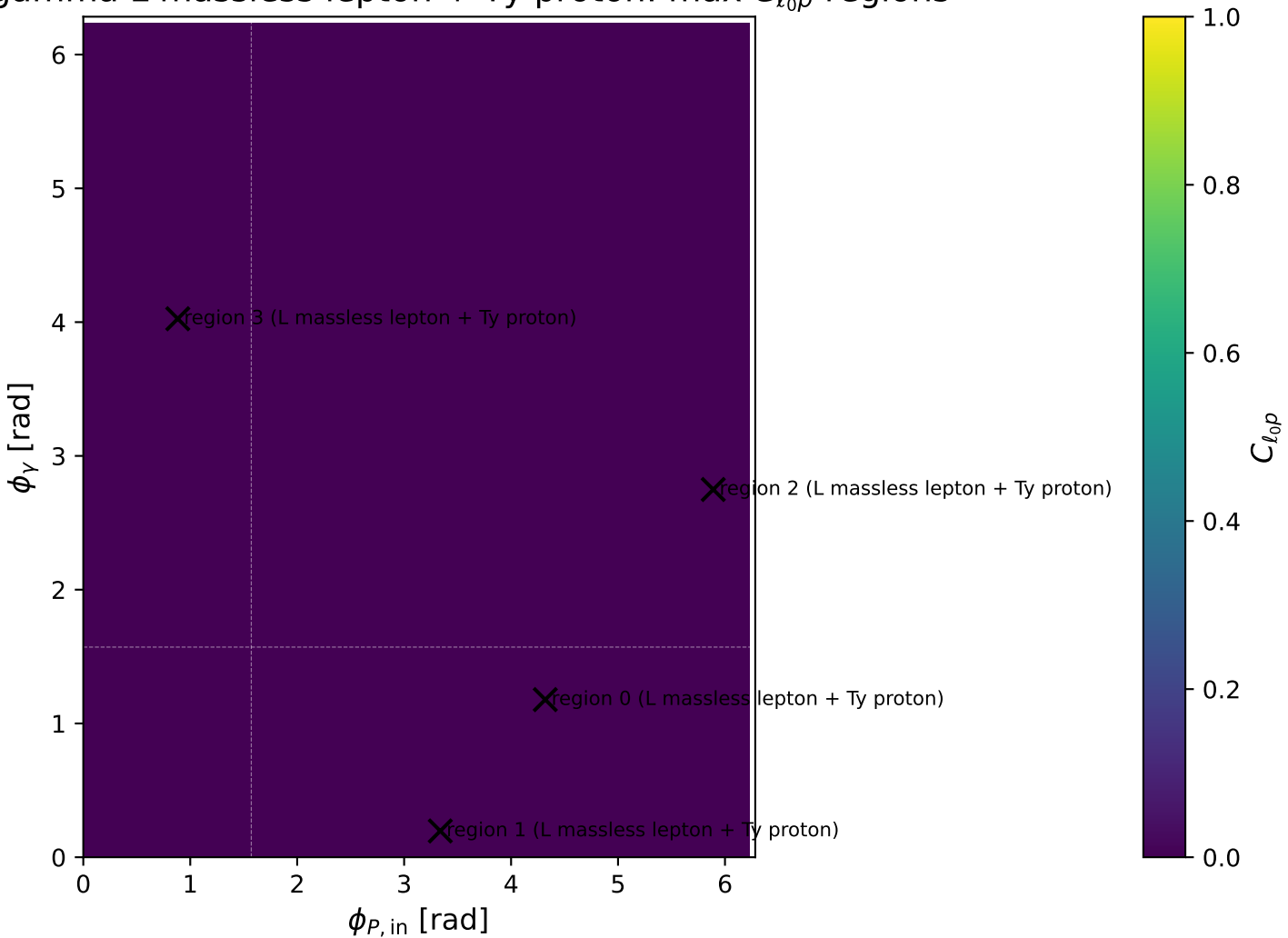
gamma L massless lepton + Ty proton: max C_{l_0p} regions
